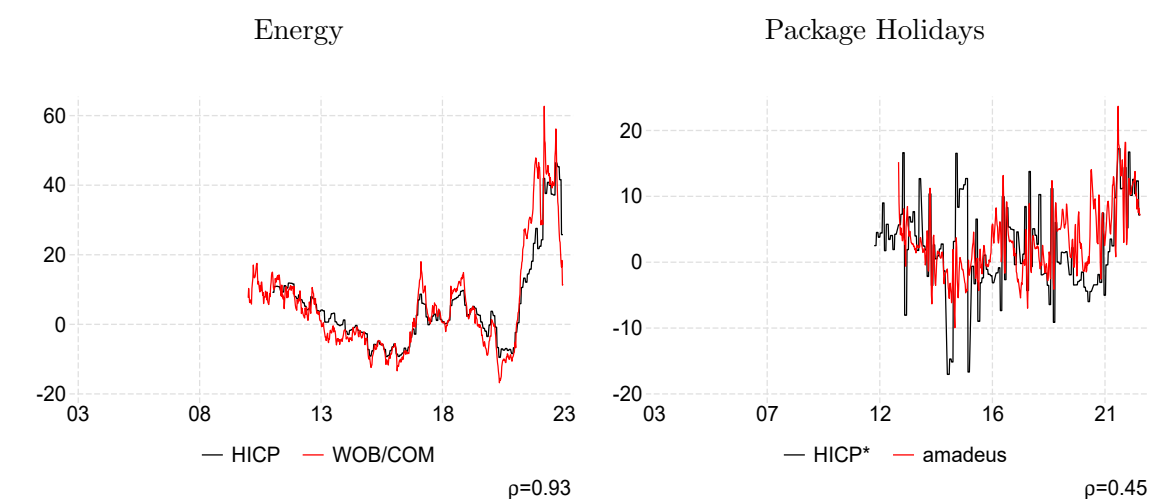
Figure A1: HICP inflation and high-frequency counterparts
