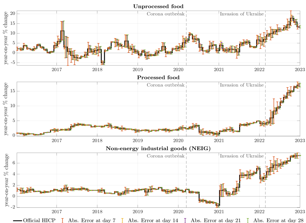
Figure C3: Absolute forecast errors over time: tracking the nowcasting performance of GfK:FMCG product groups
