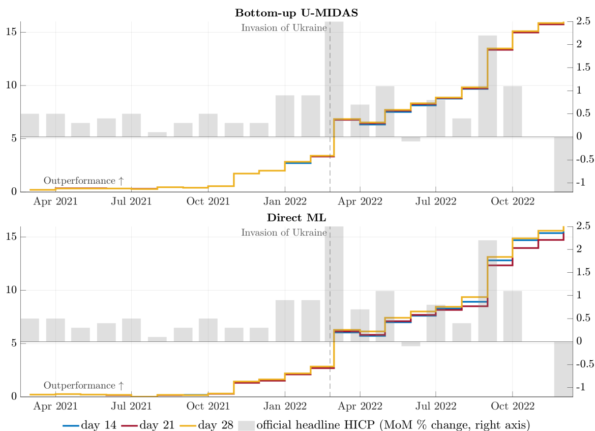
Figure C4: Cumulative sum of the squared forecast error differentials: models versus Consensus market expectations
