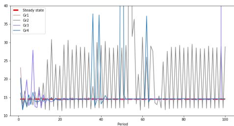
(c) \lambda = 3.8
