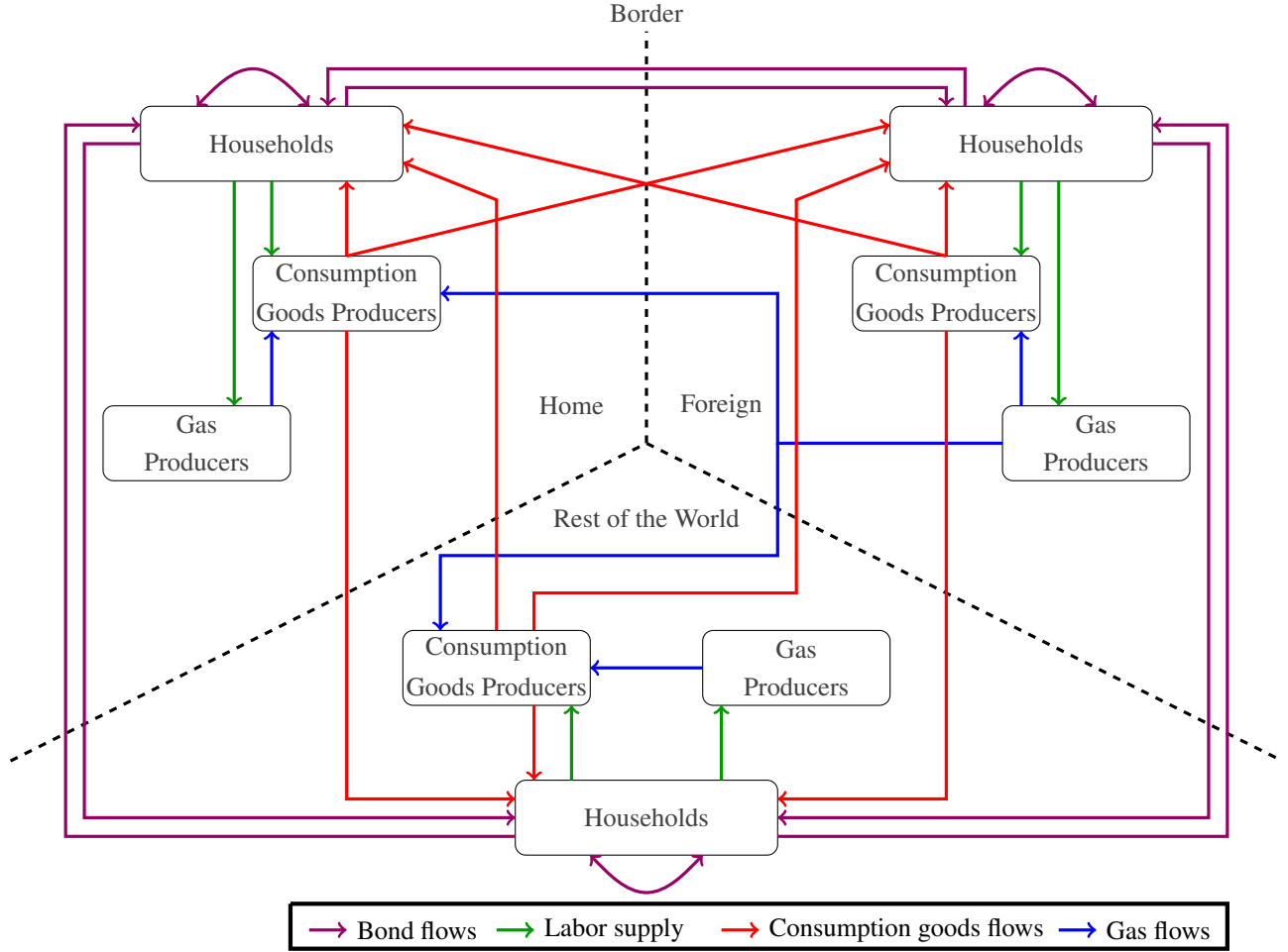
Figure 1: Model Architecture
