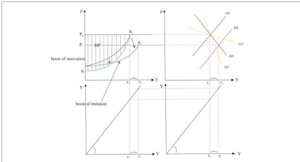
Figure 2. Innovations, imitations, output (Y) and the price level (P).
