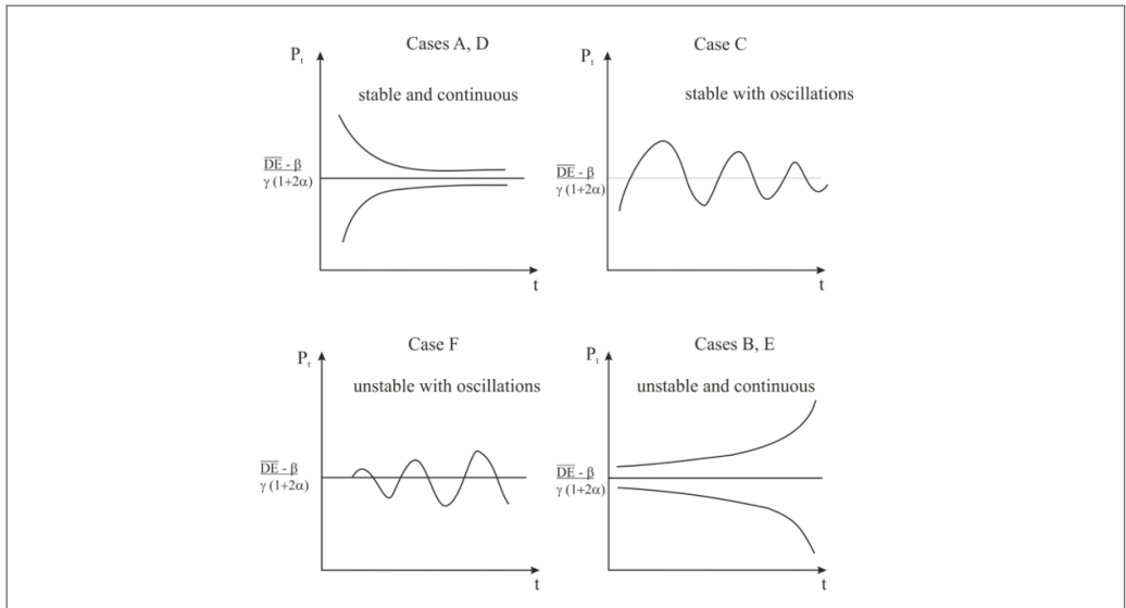
Figure 5. Stable/unstable and steady/oscillating development of prices in the Barone's Curve Model.
