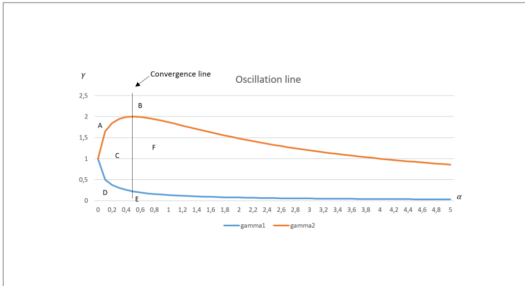
Figure 4. Oscillation and convergence lines in the dynamic Barone’s Curve Modell.
