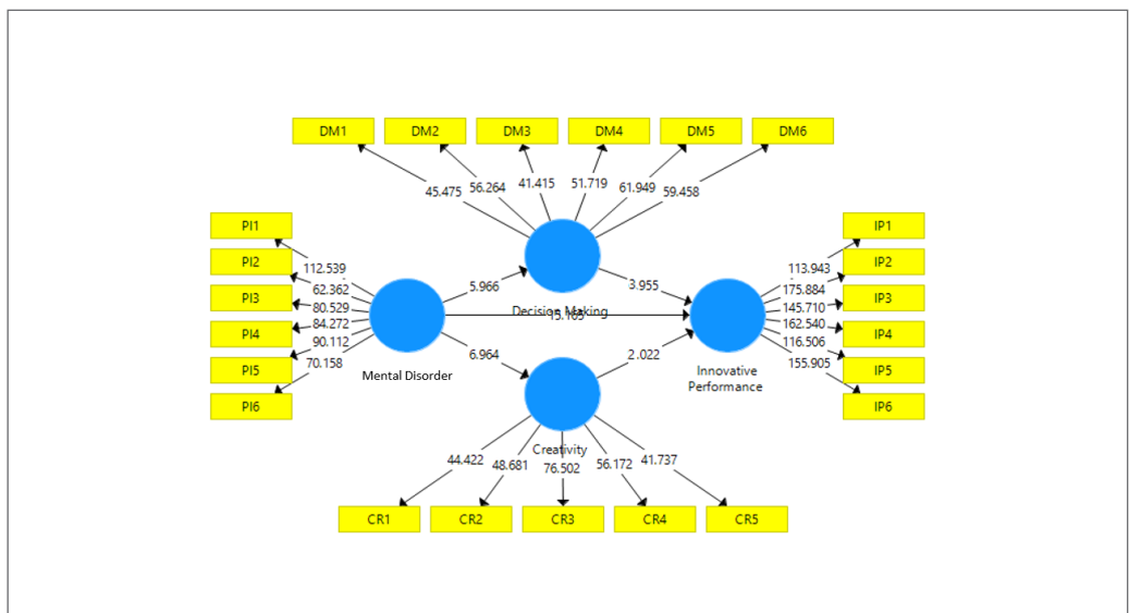
Figure 4. PLS-structural model.
