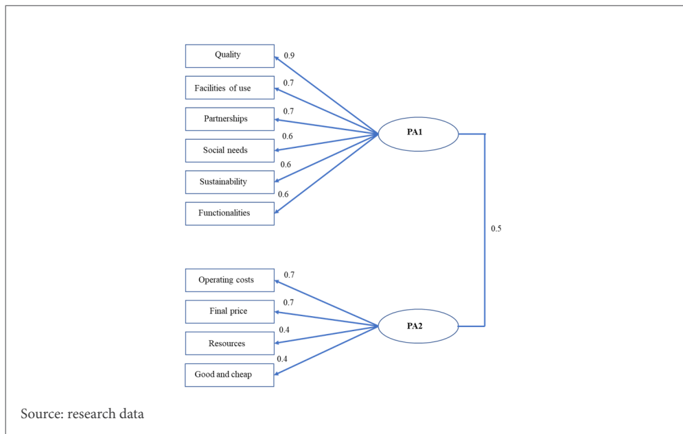
Figure 5 Factor Loadings
