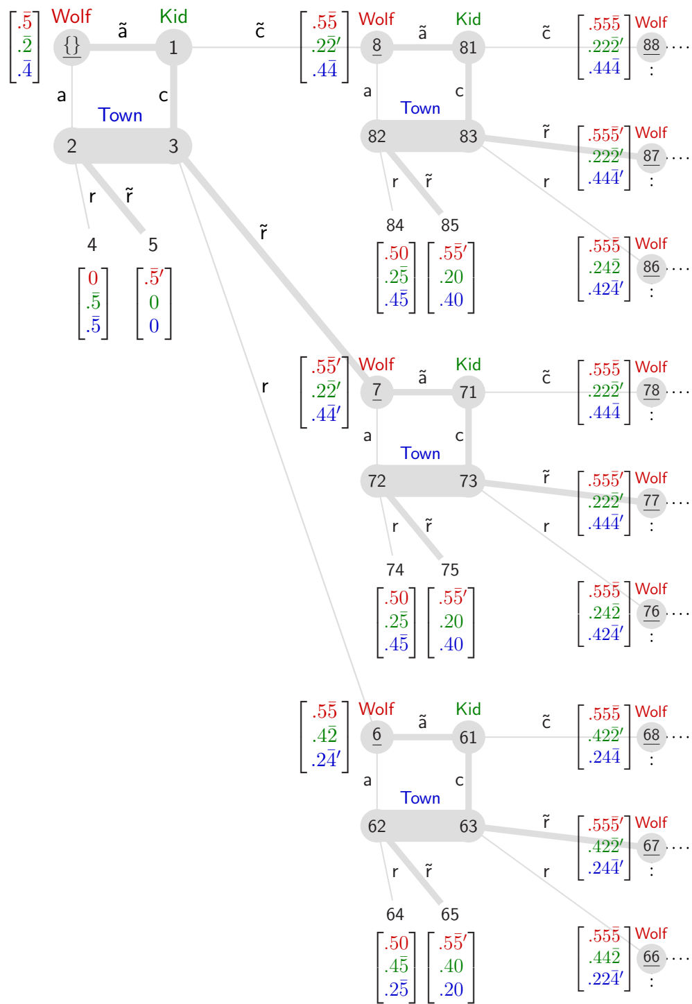
FIGURE 2.4. A strategy shown by the heavy edges, and a value function shown by the value profiles at the subroots (subroots are underlined).
