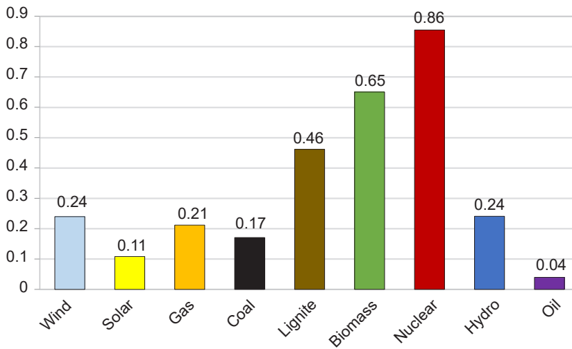
Figure 4: Load factor of each power source
