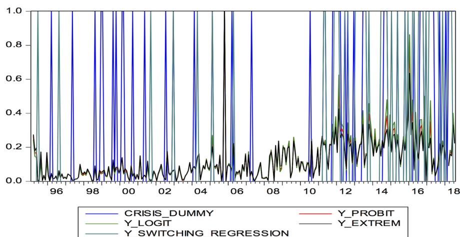
Fig. 2. In-sample and out-sample forecasts for different models.
