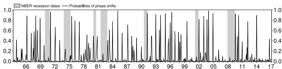
Fig. 4. Probabilities of the small caps to transition with a delay.
