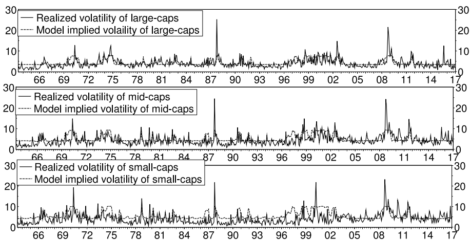
Fig. 2. Comparison of volatilities implied by the model and realized volatilities.
