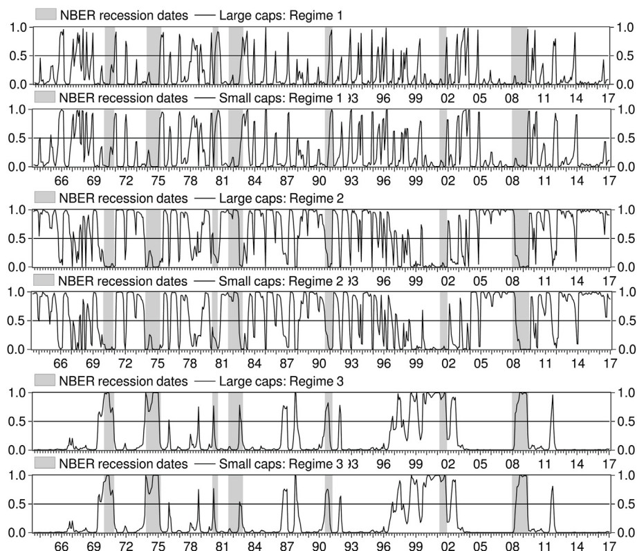
Fig. 1. Posterior probabilities of regimes of LC and SC.
