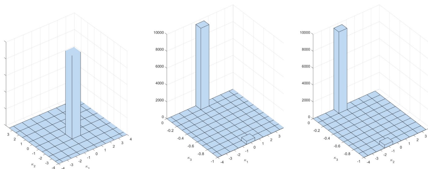
Fig. 3. Bivariate histograms of lead/lag times for LC and SC regimes.
