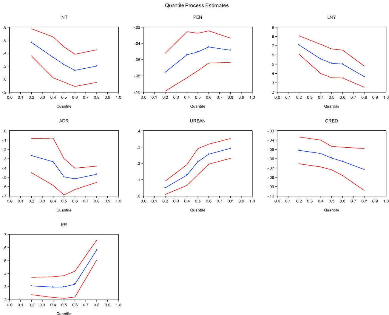
Fig. 1. Dynamics of panel quantile regression coefficients Note: The red lines indicate the 90% confidence interval, while the blue lines show the coefficients.
