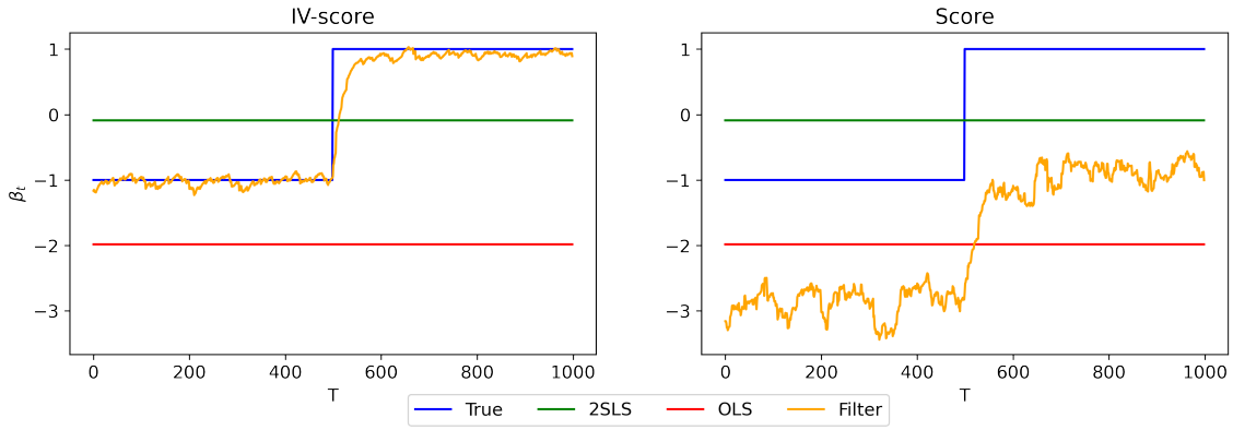
Figure 5: \beta_t with a midway break (DGP 4).
