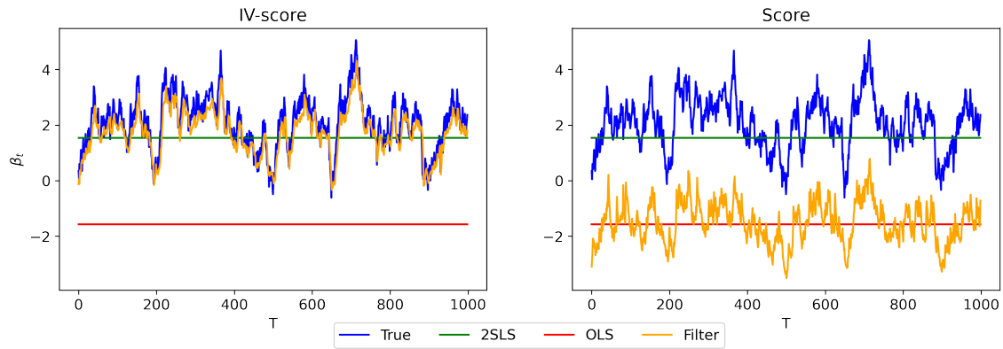
(b) h_t with a midway break (DGP 3).
