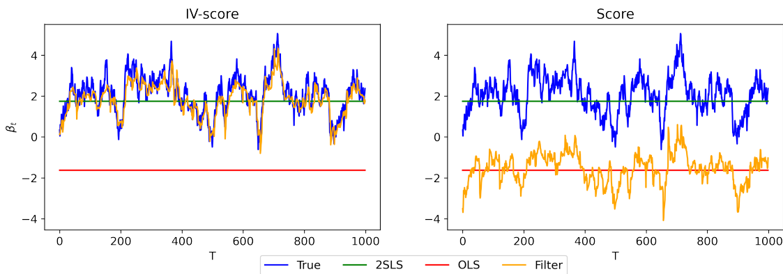
Figure 1: Estimated paths of the causal parameter with DGP 1 where h_t follows an AR(1).
