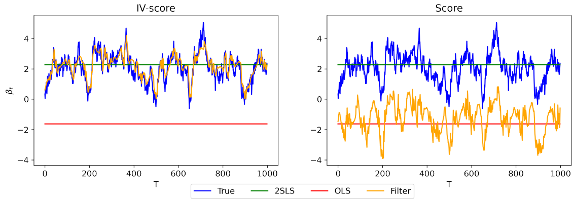
(a) h_t following sine dynamics (DGP 2).
