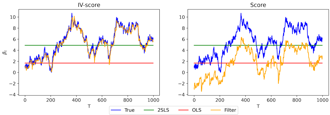
Figure 6: \beta_t following a random walk (DGP5).
