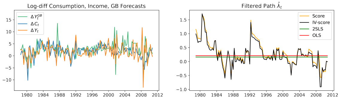
Figure 3: Data and filtered path of excess sensitivity parameter \lambda_t
