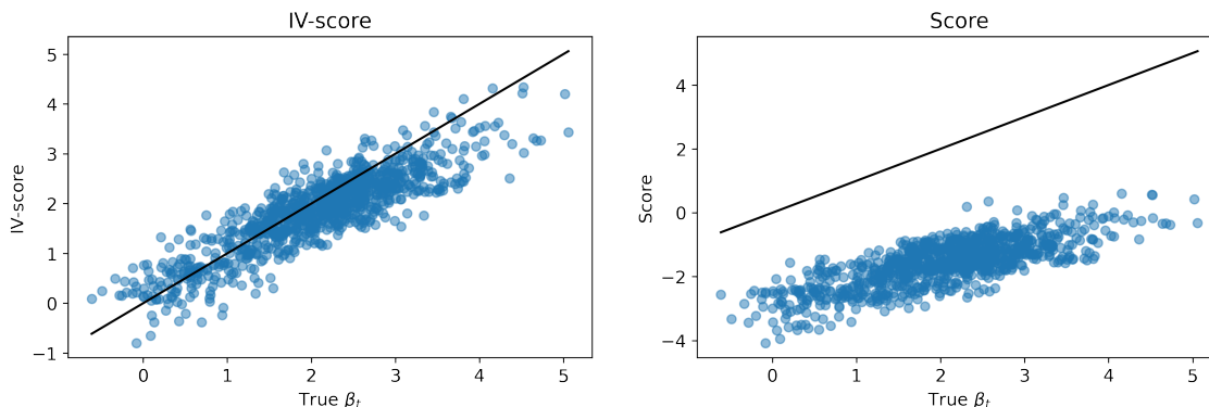
Figure 2: Scatter plot of IV-score and score filtered values vs. true \beta_t for DGP 1 where h_t follows a sine function.
