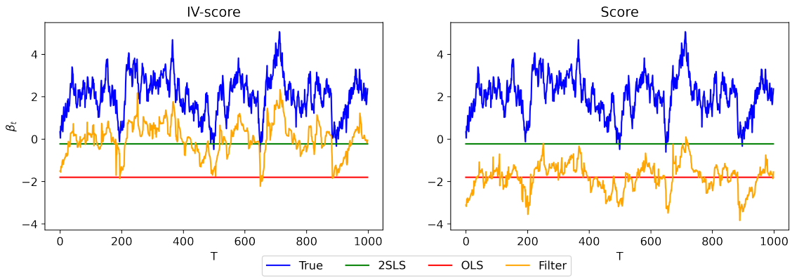
Figure 7: Filtering with an endogenous instrument (DGP 6).
