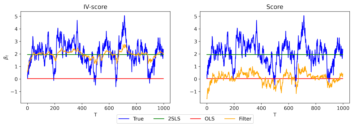
Figure 8: Filtering with large error variance (DGP7).
