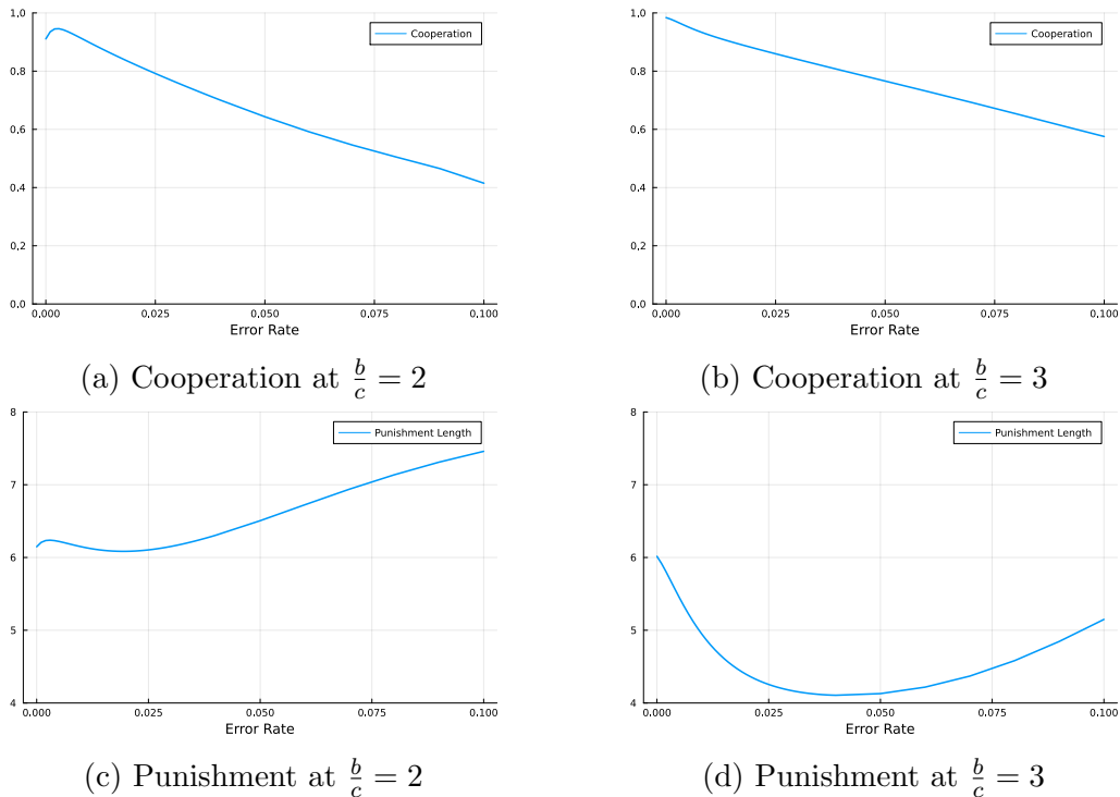
Figure 23: Cooperation and punishment in the reduced model as a function of the error rate. The level of cooperation in panels (a) and (b) is calculated as the weighted sum of the proportions at which the individual strategies, S_0 to S_{20} and All D, as residents play cooperate at a given \epsilon . The weights reflect the proportion of time the population spends with the respective strategy as a resident, and are calculated like in Figure 21 as the strategies' weights in the stationary distribution of a Moran process, where mutations happen with uniform probability between all strategies in the reduced strategy set, and where the mutation rate is infinitesimally small. Analogously, the punishment length in panels (c) and (d) is calculated as a weighted sum of expected (discounted) punishment lengths of the individual strategies. For strategy S_n the expected punishment length is computed as \frac{1-\delta^n}{1-\delta} . As in Figure 24, All D is not considered in this weighted sum, and the weights of all remaining strategies are normalised to add up to one. The continuation probability is \delta = 0.9 .
