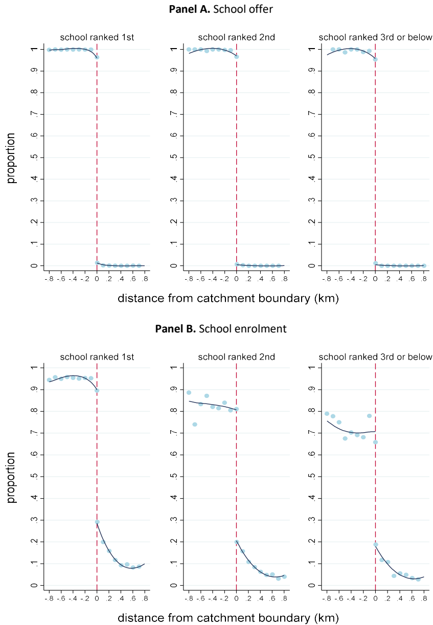
Figure C.3: Tie-breaking
