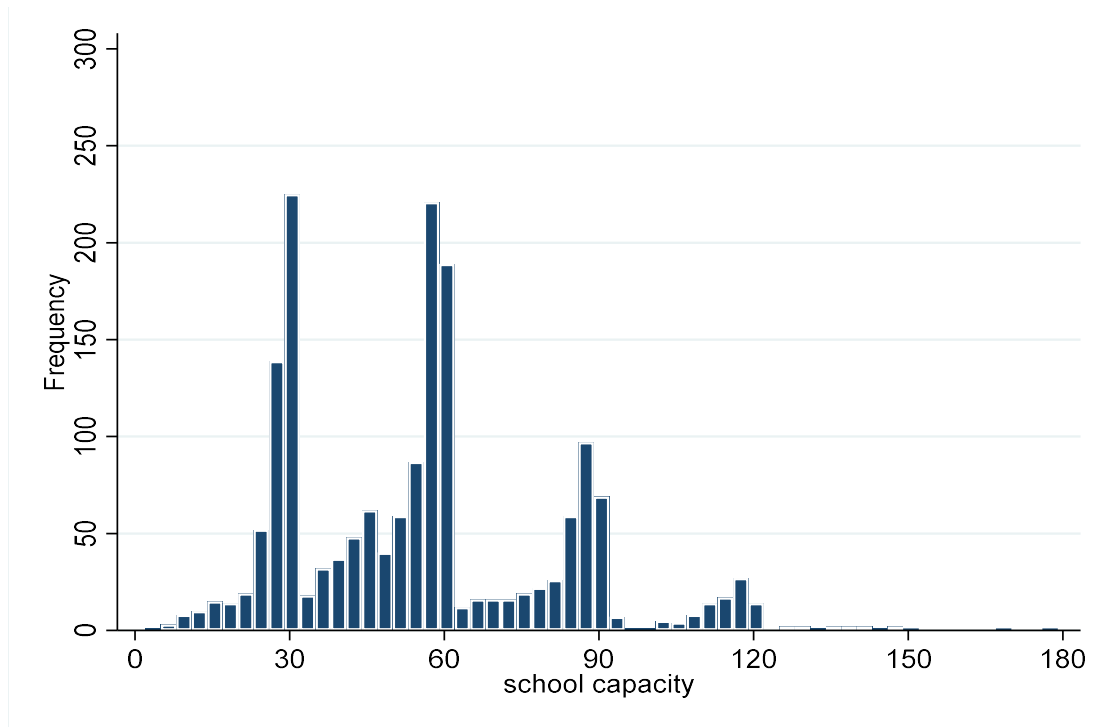
Figure C.1: School capacity
