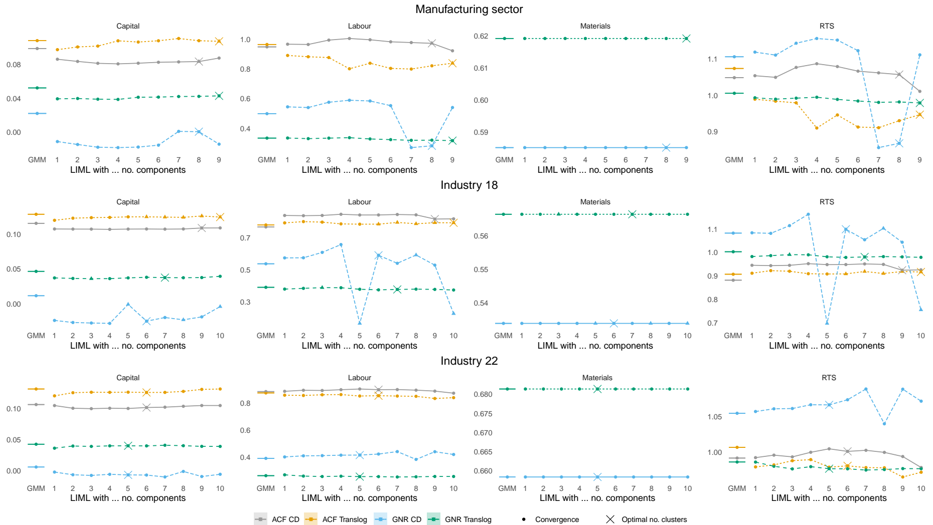
Figure D.2: Change in output elasticities, based on Akerberg et al. (2015) and Gandhi et al. (2020) Cobb-Douglas and Translog production function estimators with endogenous labor, in function of the number of clusters for the entire manufacturing sector and industries 18 and 22 of the Belgian economy.
