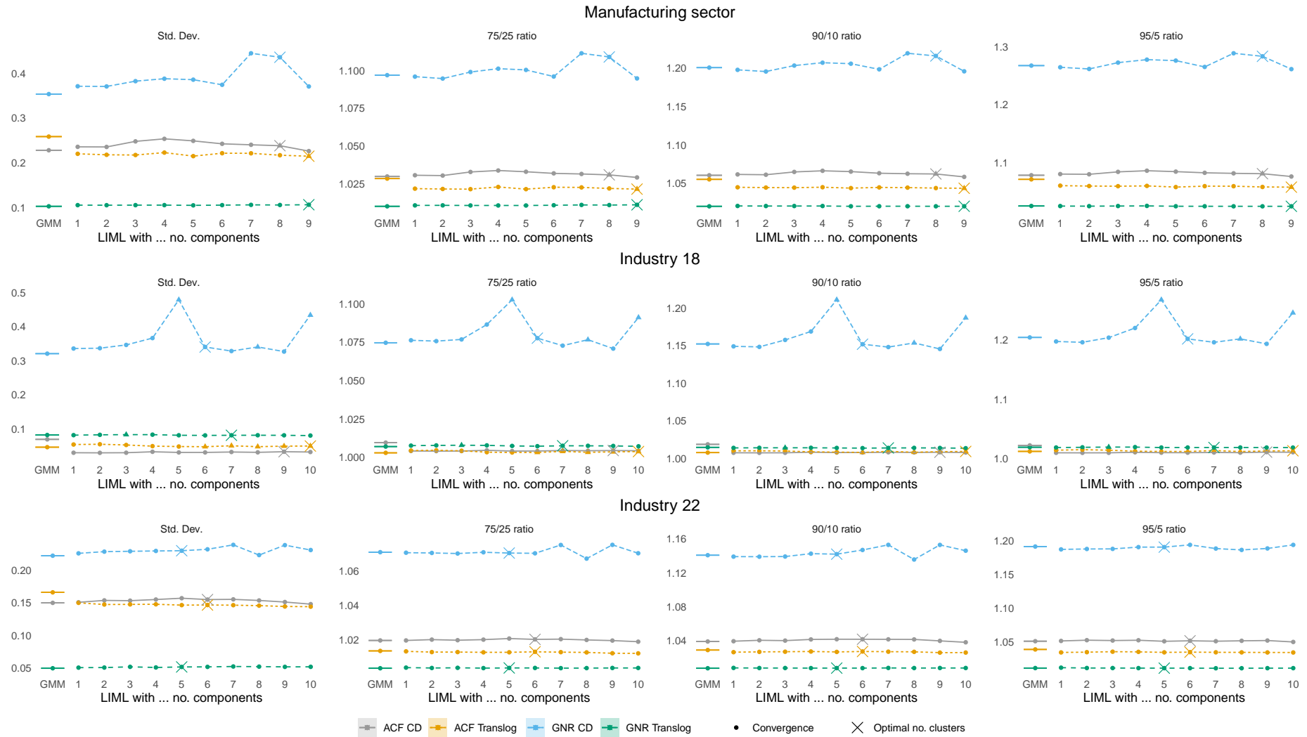
Figure D.4: Change in the standard deviation, 75/25-, 90/10-, and 95/5-ratio, based on Akerberg et al. (2015) and Gandhi et al. (2020) Cobb-Douglas and Translog production function estimators with endogenous labor, in function of the number of clusters for the entire manufacturing sector and industries 18 and 22 of the Belgian economy.
