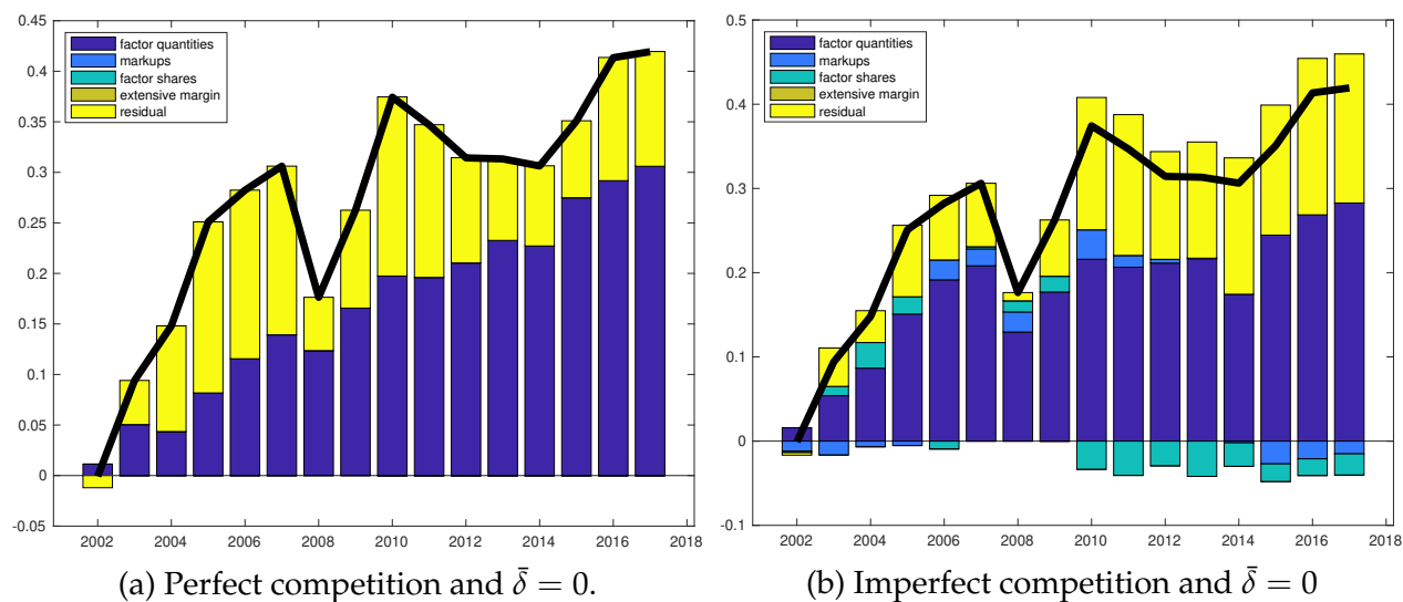
Figure 3: Growth accounting special cases
