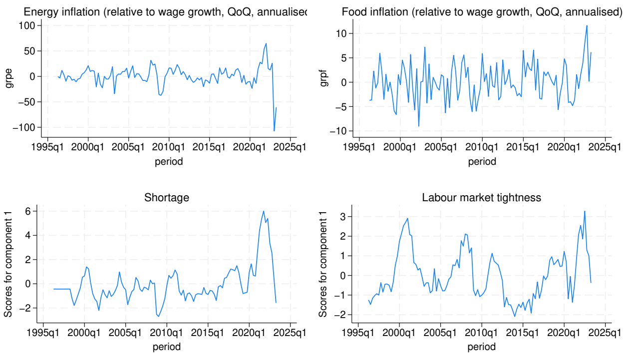
Figure 10: Data plots - main exogenous variables.
