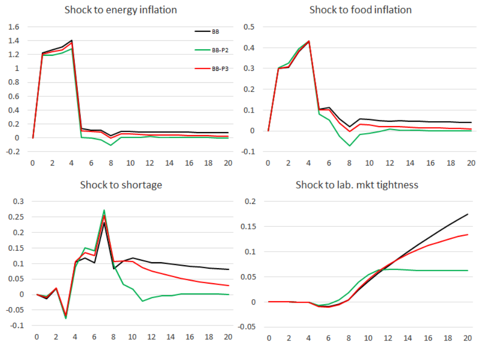
Figure 16: Impulse responses of Belgian consumer price inflation (NICP, year-on-year ).
