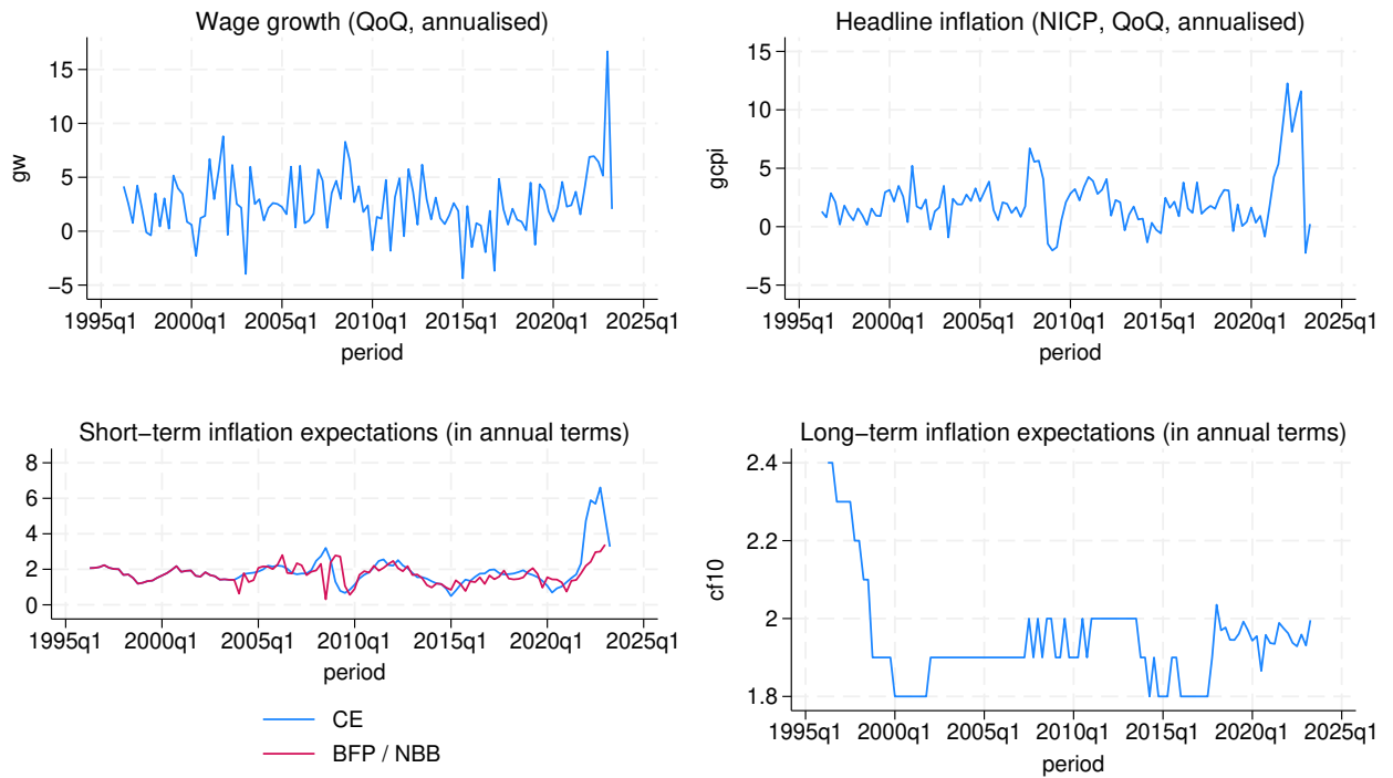
Figure 9: Data plots - endogenous variables.
