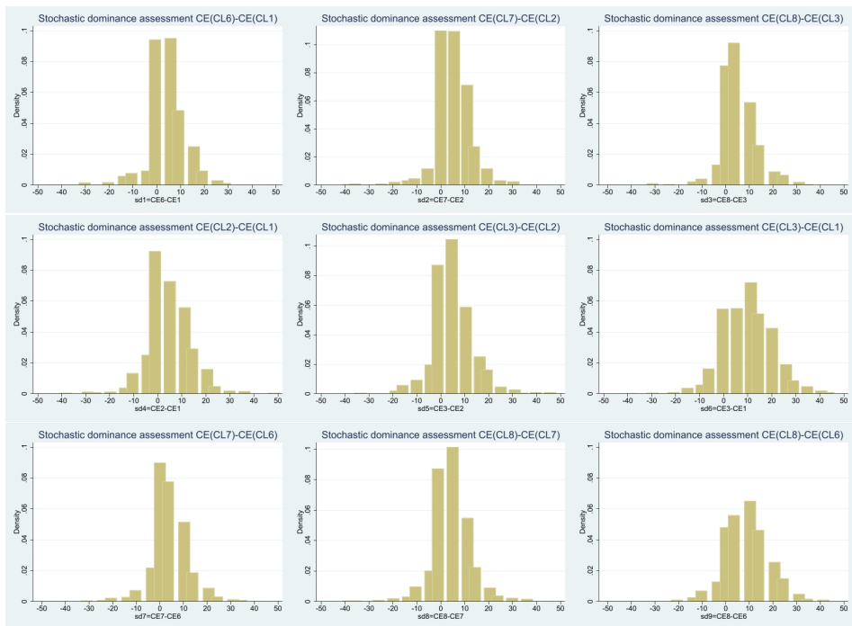
Fig. 5 Stochastic dominance assessment with value deviations
