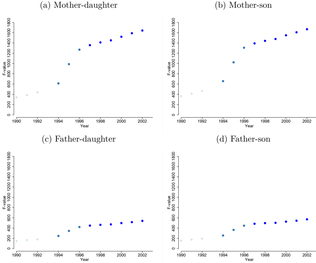
Figure D.4: F statistic from first stages
