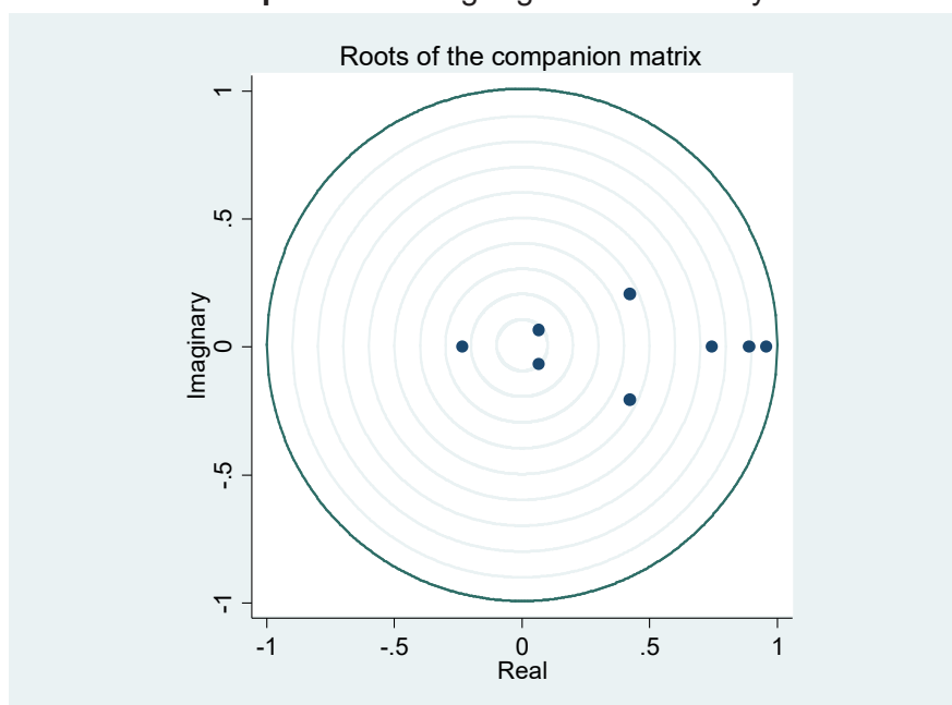
Graph 5. Checking Eigenvalue Stability
