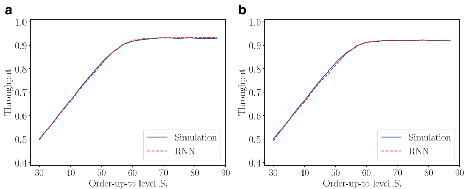
Fig. 6 Throughput of 4- and 6-machine lines with processing rate \mu_i = 1TU^{-1} , buffer size C_i = 20 and length of the replenishment interval r = 60TU with variation in order up-to level S_i predicted via RNN and simulation. a 4-machine line, b 6-machine line
