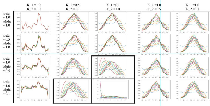
Fig. 4 Sensitivity analysis in the close boundary. The random seeds, based on a uniform distribution, were set to obtain the same initial arrays. Subfigures in lines show variations in the scale parameters, and columns show variations in the size parameters. Different colors in each plot represent iterations, starting from a uniform distribution. The model validation uses the parameters K_1 = 0.1 , K_2 = 1.0 , \beta = 1.0 , and \alpha = 0.3
