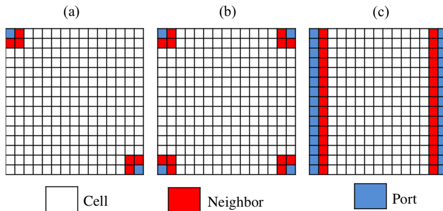
Fig. 3 Port configurations. Subfigure a is the basic two ports; subfigure b is the corner configuration; and subfigure c is the lateral configuration
