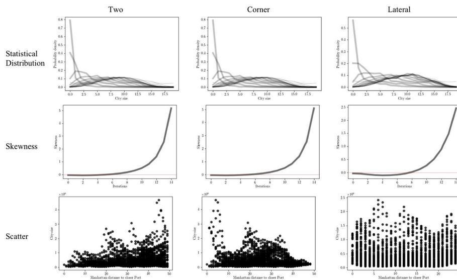
Fig. 7 Port configurations. Dynamics of the statistical distributions, skewness, and correlations. The skewness was computed by the Fisher-Pearson coefficient scipy.stats.skew . Each value of skewness is associated with each curve of statistical distribution per case. Scatter plots: (x-axis = Manhattan distance to closer port, y-axis = city-size)
