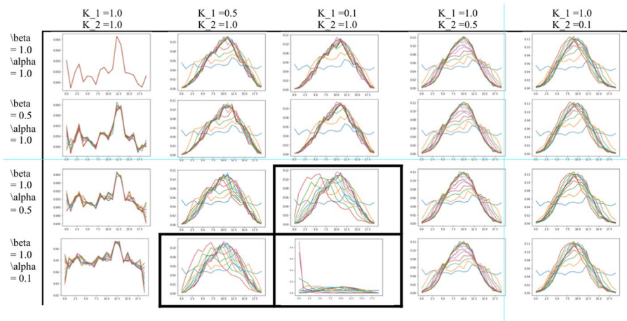
Fig. 5 Sensitivity analysis in the open boundary. The random seeds, based on a uniform distribution, were set to obtain the same initial arrays. Subfigures in lines show variations in the scale parameters, and columns show variations in the size parameters. Different colors in each plot represent iterations, starting from a uniform distribution. The model validation uses the parameters K_1 = 0.1 , K_2 = 1.0 , \beta = 1.0 , and \alpha = 0.3
