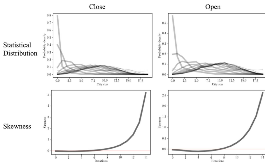
Fig. 6 Base cases. Dynamics of the statistical distributions and skewness. The skewness was computed by the Fisher-Pearson coefficient scipy.stats.skew . Each value of skewness is associated with each curve of statistical distribution per case
