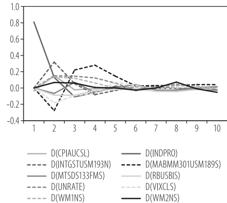
Figure 6: Response of D(INDPRO) to Innovations
