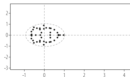
Figure 4: Inverse Roots of AR Characteristic Polynomial
