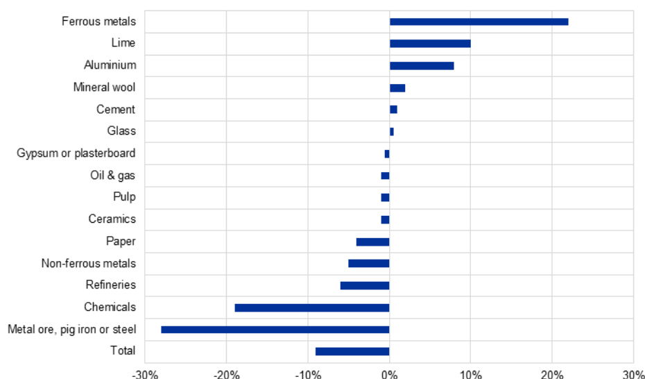
Scenario for emissions savings per sector from a carbon price-driven reallocation
