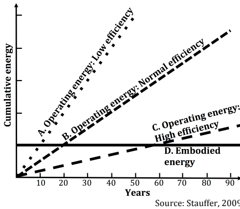
Figure 16. The changing relationship between embodied and operational energy consumption over time in buildings
