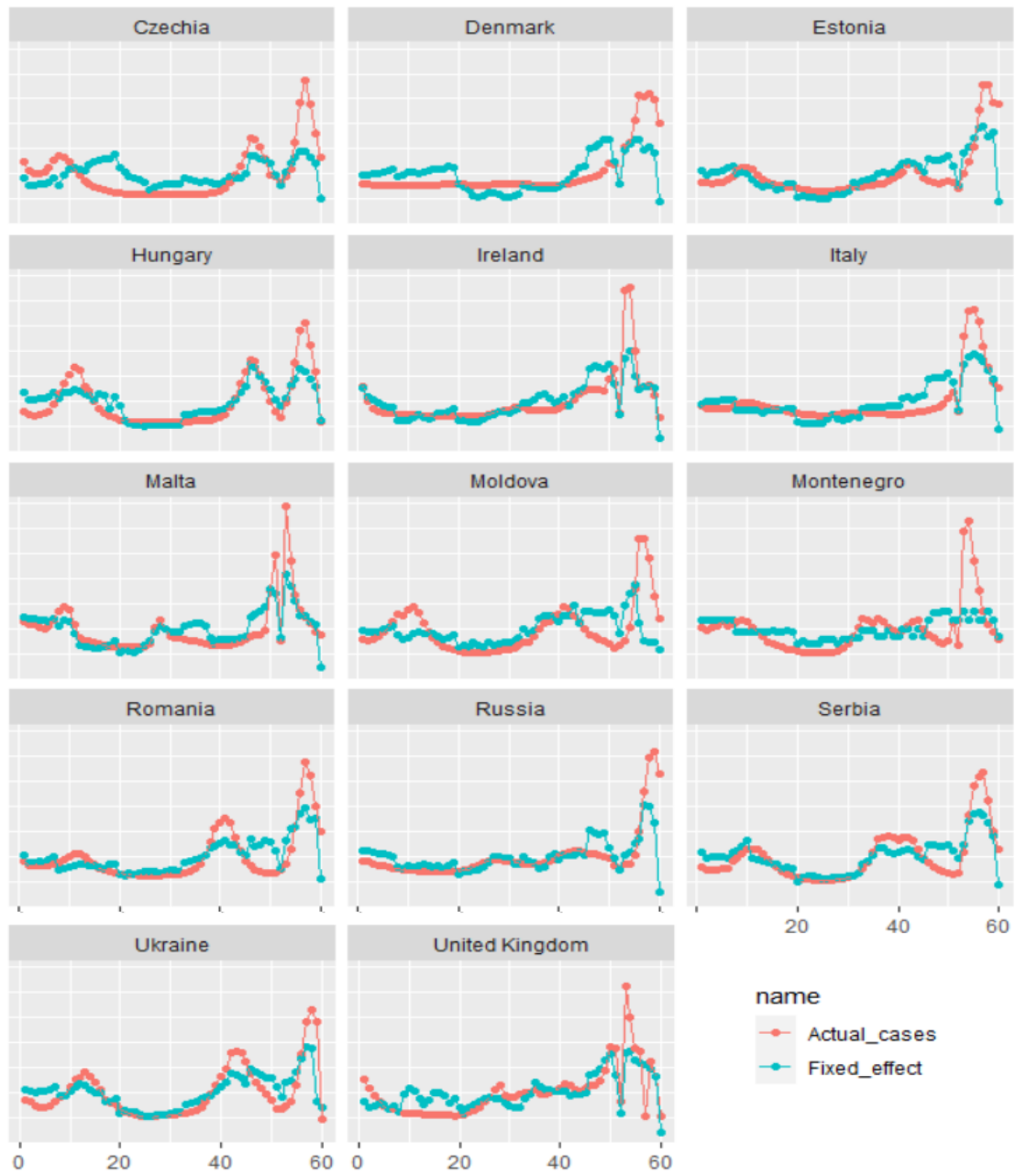
Figure 2: Actual versus fitted values (Infections) based on fixed effects estimation
