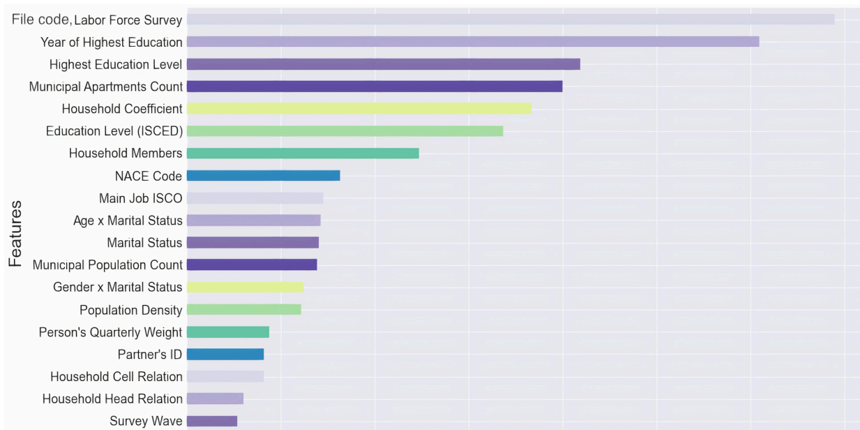
Figure 27: Top 20 Feature Importances in the Random Forest Model
