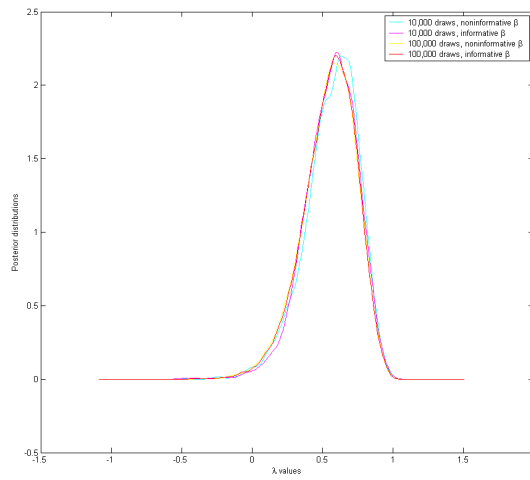
Figure 4: Density plots of estimated \lambda^1
