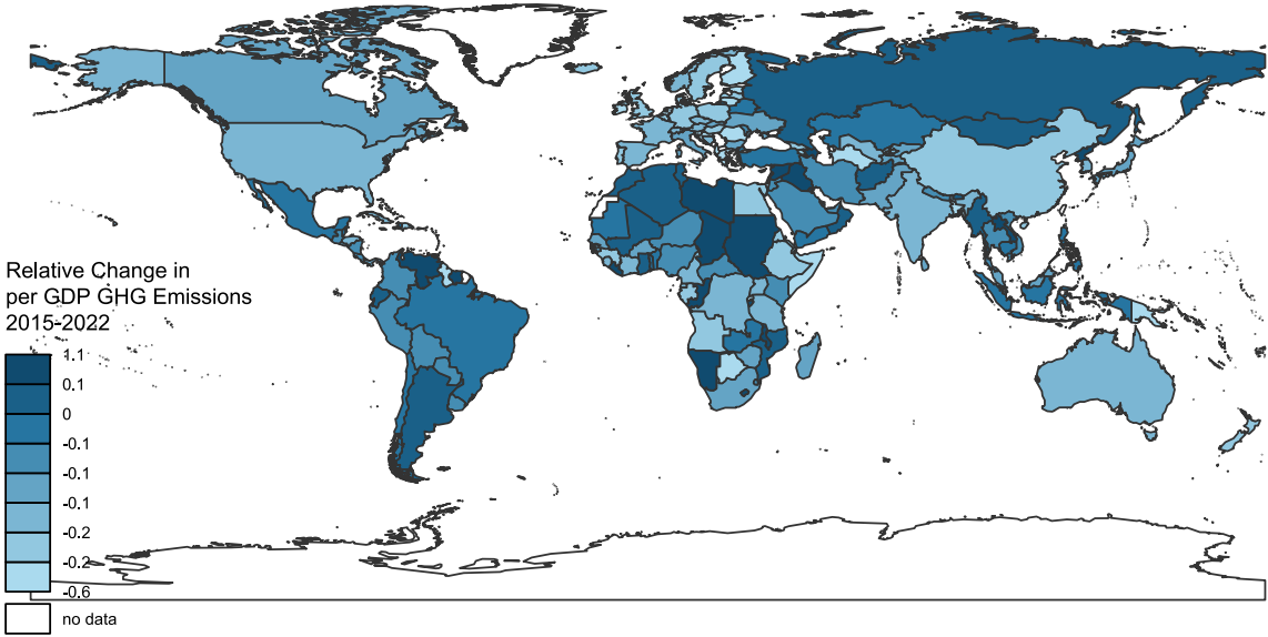
Figure 4. Overview of each country's change relative to their emission intensity rate in 2015. Each countries relative change in annual GHG emissions per GDP since 2015 is presented. Data: EDGAR
