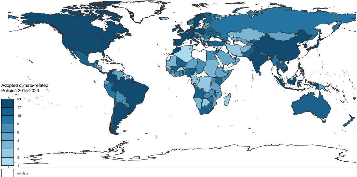
Figure 1. Number of climate-related policies adopted by each country since the Paris Agreement, covering the period when the Agreement was drafted in December 2015 to 2023. Data: CPR
