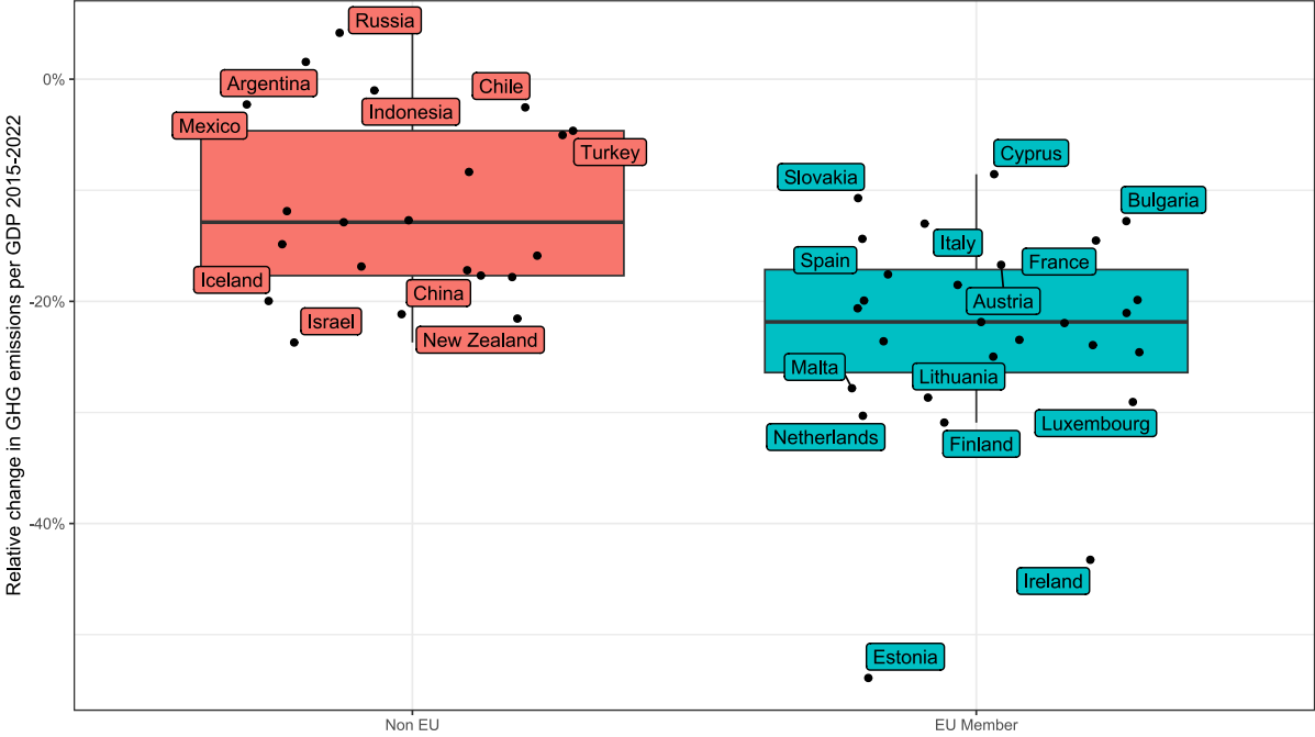
Figure 5. Overview of the relative change in GHG emissions per GDP from 2015 to 2022 for OECD/G20 members (without EU members) and EU members. The thick black line represents the median for both groups, and the colored boxes show the interquartile range, marking the area between the 25th and 75th percentile. Data: EDGAR
