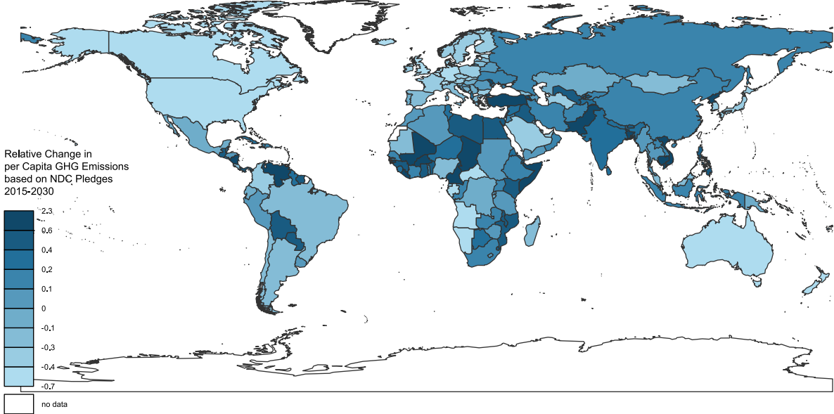
Figure 2. Overview of projected relative changes in annual GHG emissions per capita based on each country's NDC pledges and their forecasted effect on GHG per capita emissions. Data: Meinshausen et al.
