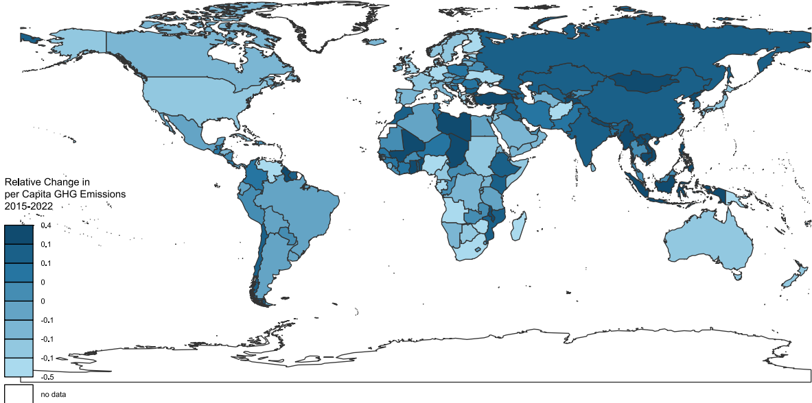
Figure 3. Overview of relative changes in annual GHG emissions per capita since the Paris Agreement. The graph presents each country's individual change in achieving climate targets. Data: EDGAR
