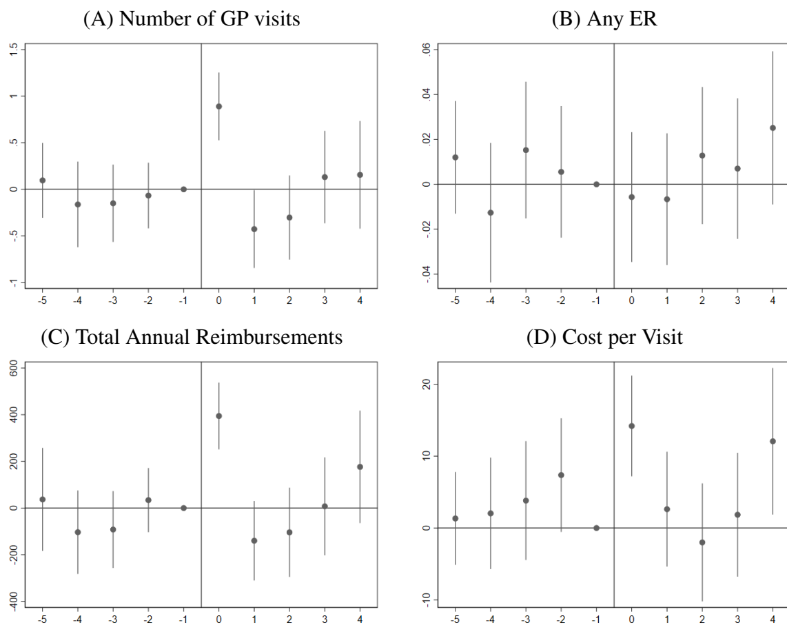
Figure A.3: Event Studies: Health Outcomes for Women with First Symptom Between 40-44 in Norway
