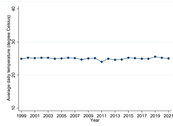
Panel A. Average daily temperature (degrees Celsius)
