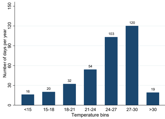
Panel A: Bins of daily temperature
