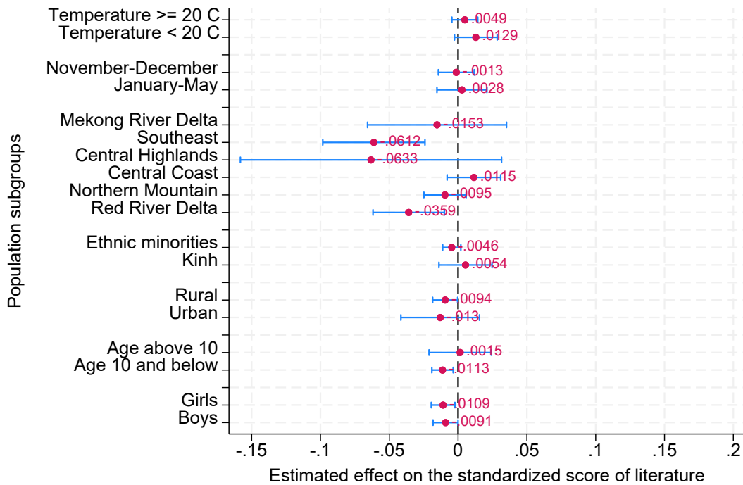
Panel B. The heterogeneous effect on the standardized reading score
