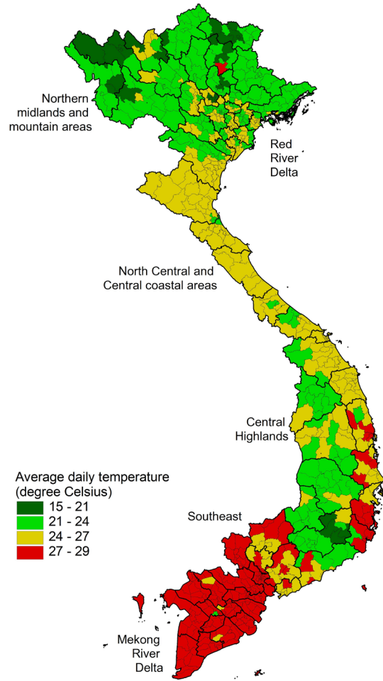
Panel A. Average daily temperature (degree Celsius)
