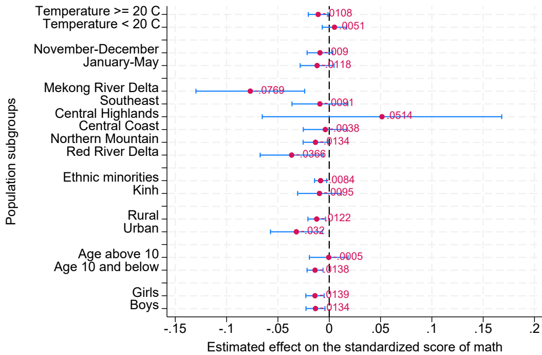
Panel A. The heterogeneous effect on the standardized math score
