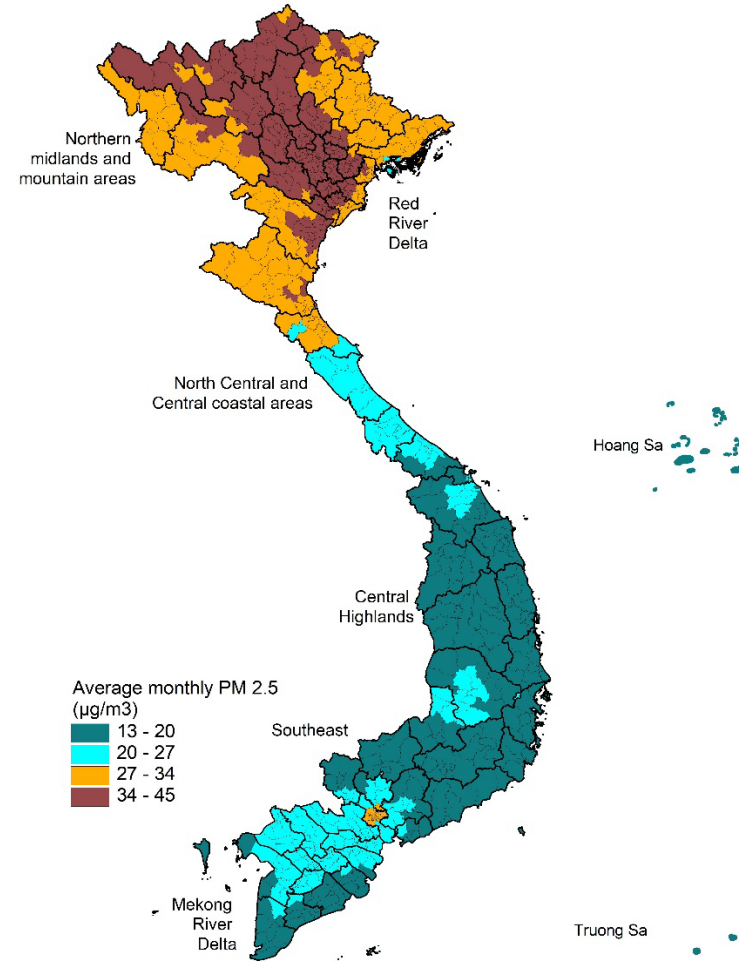
Panel B. Average monthly air pollution ( \mu\text{g}/\text{m}^3 )
