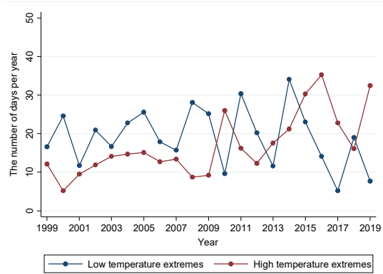
Panel B: The number of days with temperature extremes
