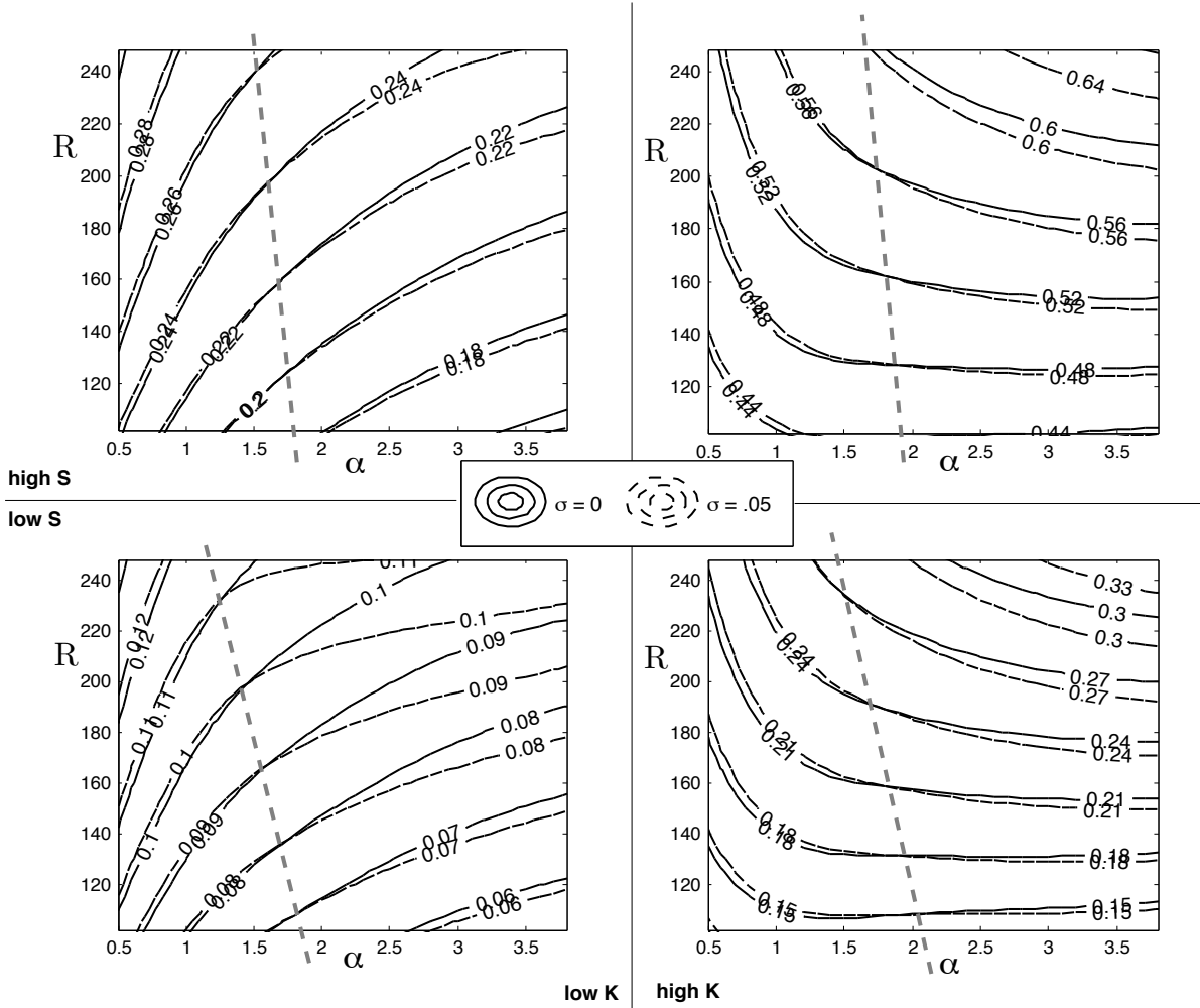
Figure 6: Optimal mitigation in \alpha - R space for different levels of \sigma and K - S combinations.
