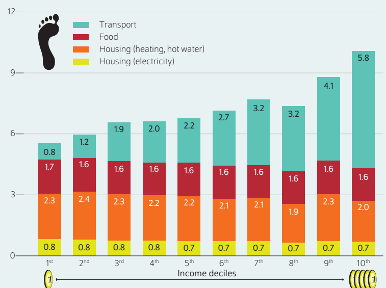
Figure 2 Per capita carbon footprint in Germany by income decile In tons of CO 2 equivalents, annual average
