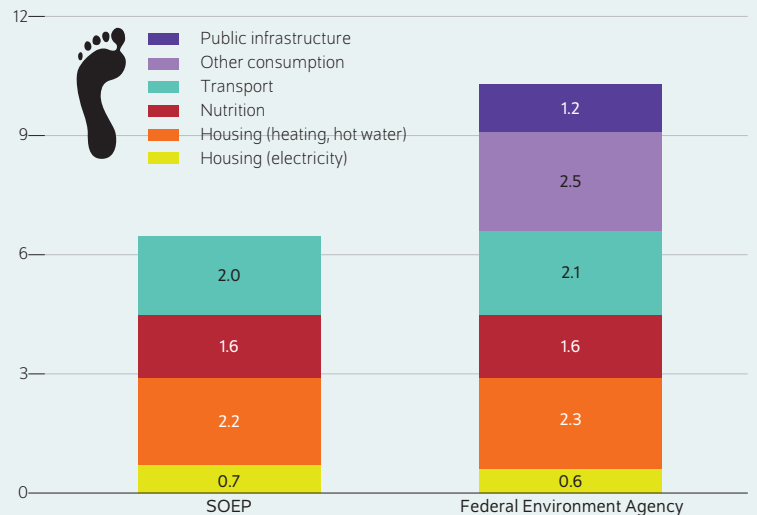
Figure 1 Greenhouse gas emissions in Germany per capita and year In tons of CO 2 equivalents
