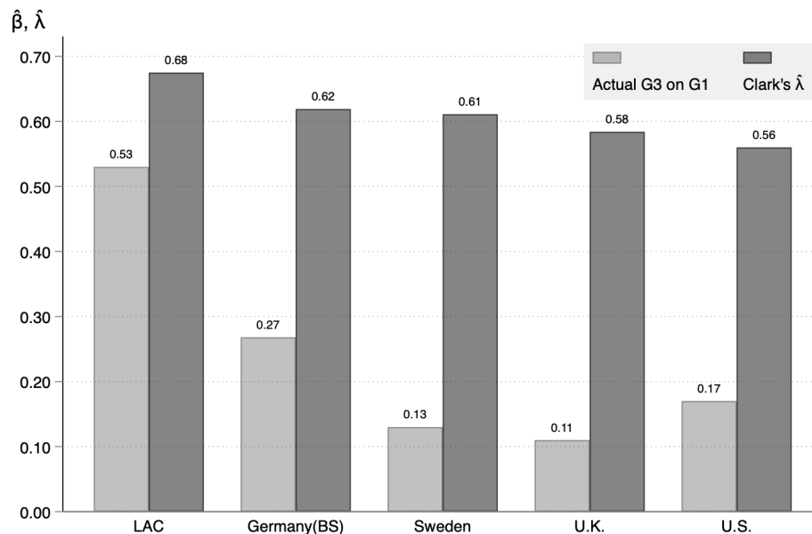
Figure 5: Actual ( \beta s) Estimates vs Clark’s Heritability Coefficient ( \lambda s)
