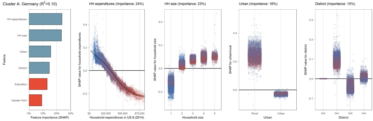
(B.9.14) Partial dependence plot (SHAP) for Germany (cluster A)
