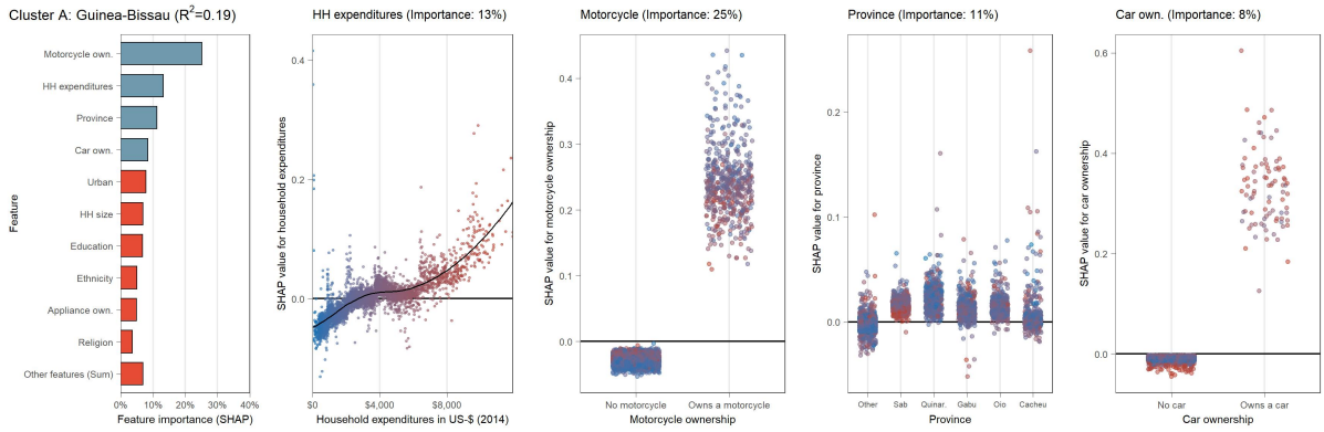
(B.9.22) Partial dependence plot (SHAP) for Guinea-Bissau (cluster A)
