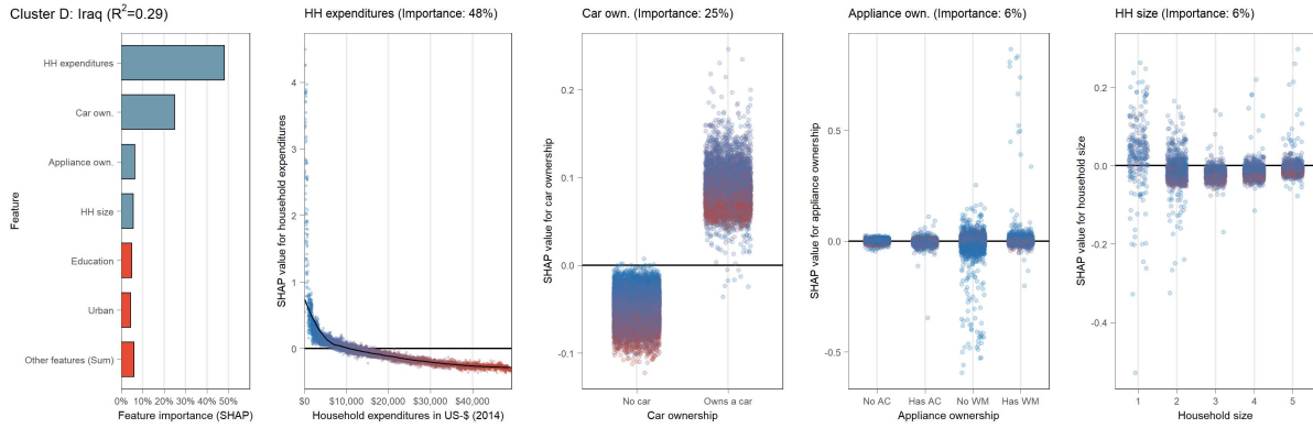
(B.9.80) Partial dependence plot (SHAP) for Iraq (cluster D)
