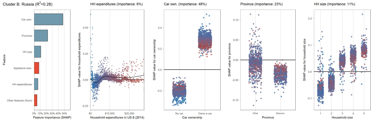
(B.9.61) Partial dependence plot (SHAP) for Russian Federation (cluster B)
