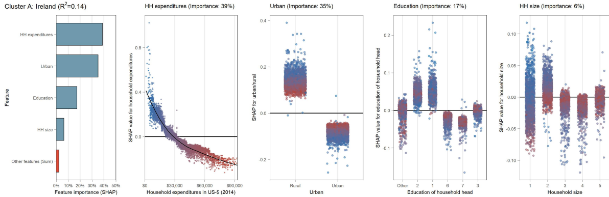
(B.9.26) Partial dependence plot (SHAP) for Ireland (cluster A)
