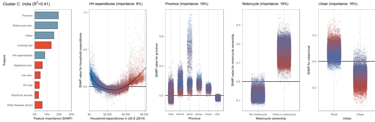
(B.9.71) Partial dependence plot (SHAP) for India (cluster C)
