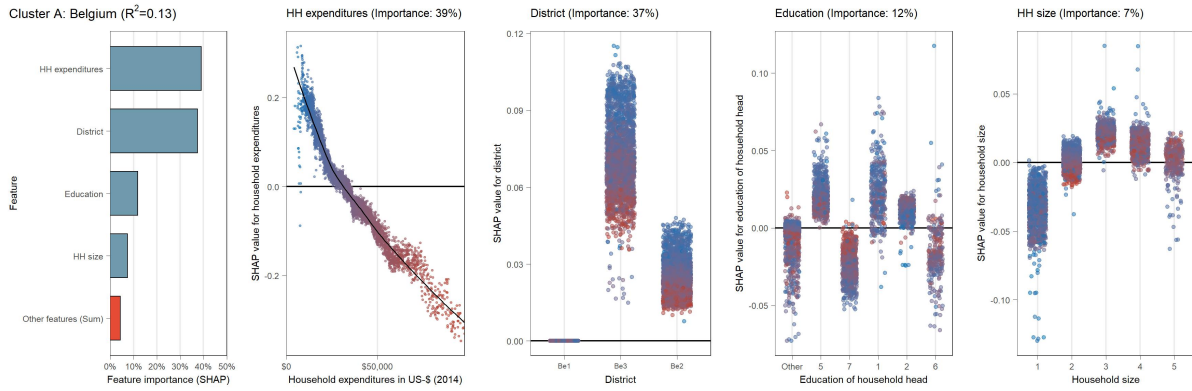
(B.9.4) Partial dependence plot (SHAP) for Belgium (cluster A)
