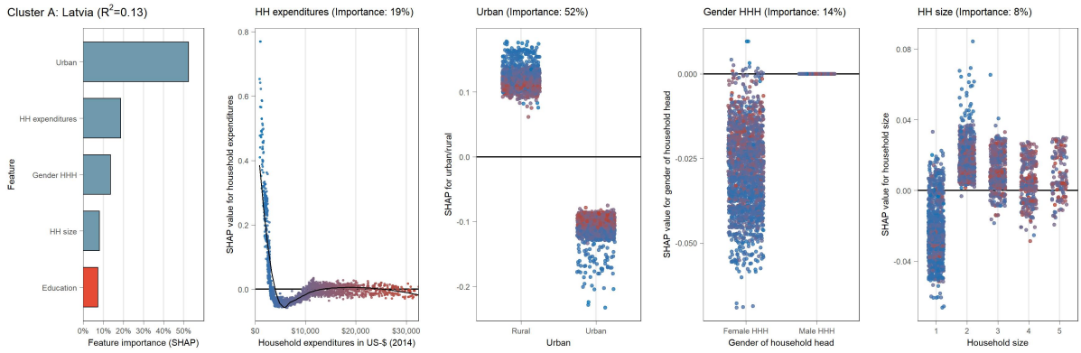
(B.9.34) Partial dependence plot (SHAP) for Latvia (cluster A)
