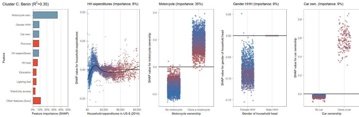
(B.9.67) Partial dependence plot (SHAP) for Benin (cluster C)
