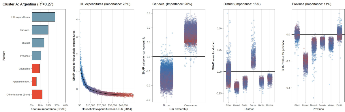
(B.9.2) Partial dependence plot (SHAP) for Australia (cluster A)
