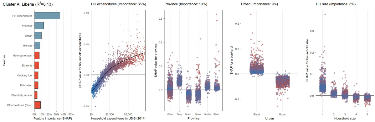
(B.9.31) Partial dependence plot (SHAP) for Liberia (cluster A)
