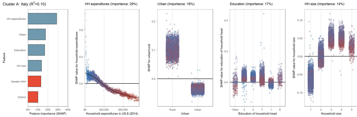
(B.9.28) Partial dependence plot (SHAP) for Italy (cluster A)
