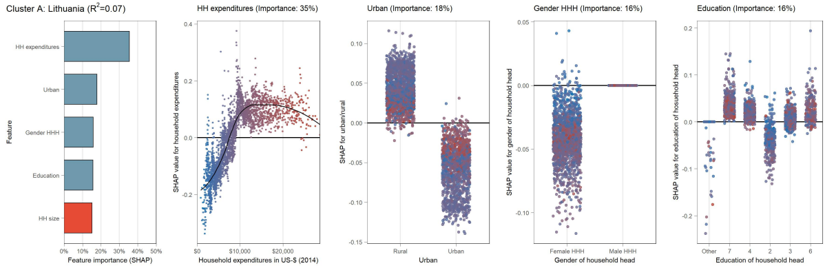
(B.9.32) Partial dependence plot (SHAP) for Lithuania (cluster A)
