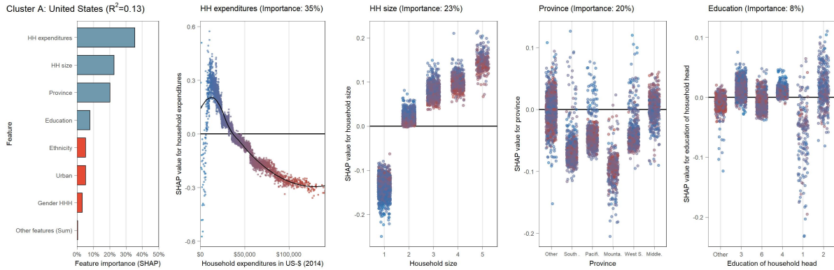
(B.9.50) Partial dependence plot (SHAP) for USA (cluster A)
