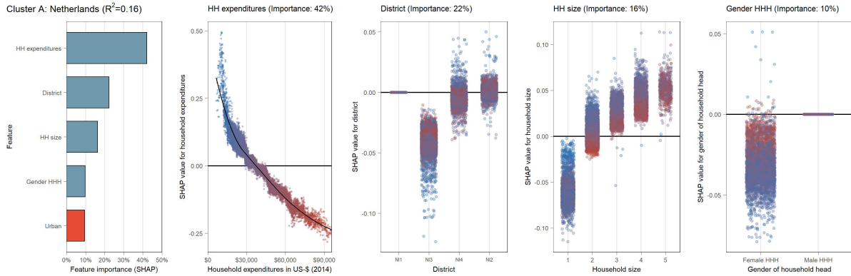
(B.9.41) Partial dependence plot (SHAP) for the Netherlands (cluster A)
