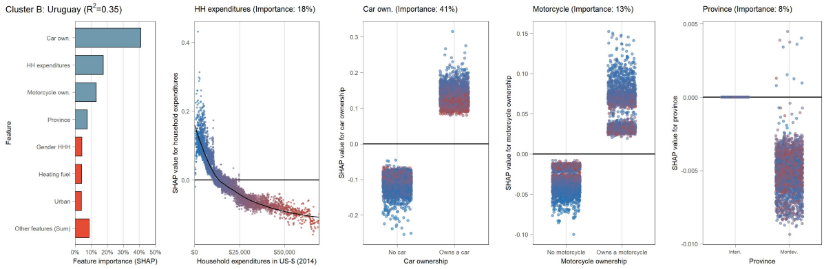
(B.9.64) Partial dependence plot (SHAP) for Uruguay (cluster B)
