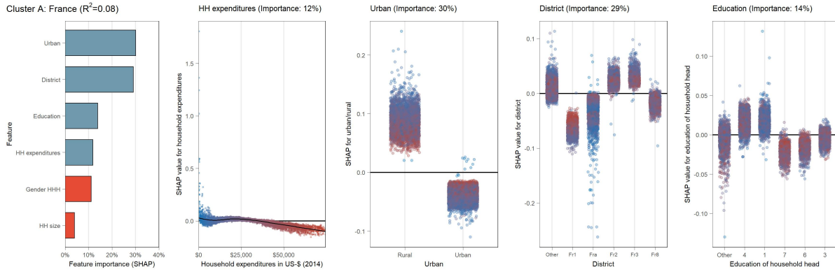
(B.9.20) Partial dependence plot (SHAP) for France (cluster A)
