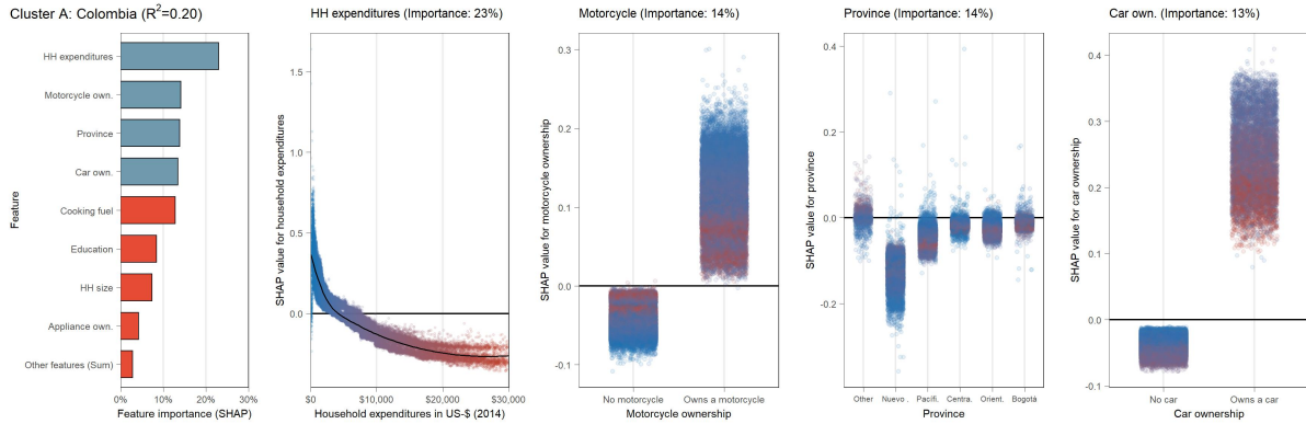
(B.9.11) Partial dependence plot (SHAP) for Colombia (cluster A)
