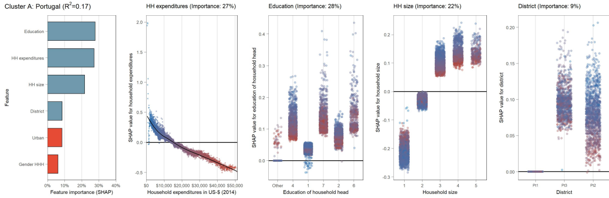
(B.9.44) Partial dependence plot (SHAP) for Portugal (cluster A)
