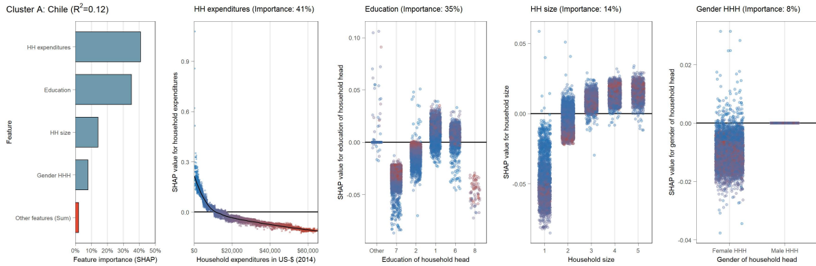
(B.9.10) Partial dependence plot (SHAP) for Chile (cluster A)
