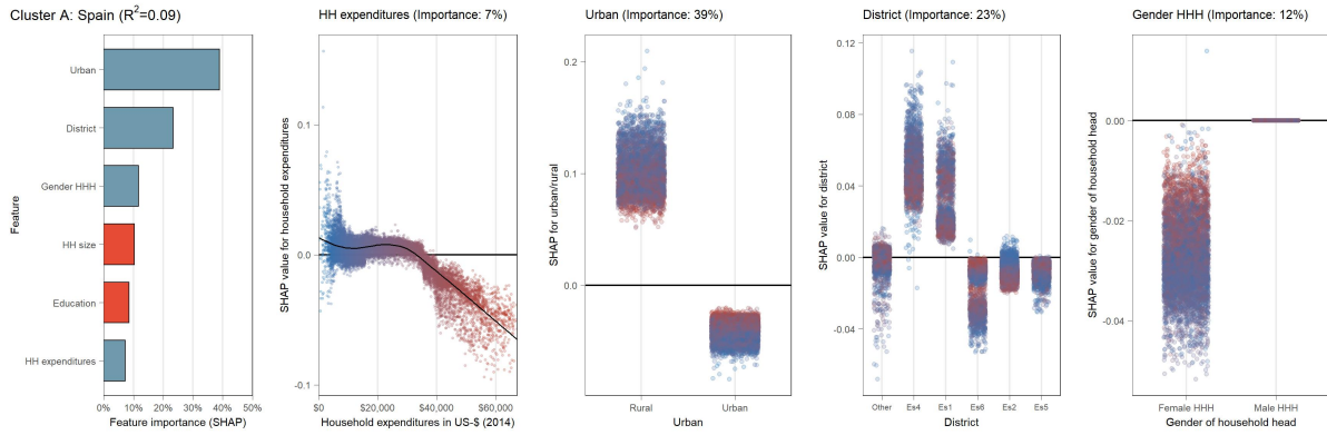
(B.9.16) Partial dependence plot (SHAP) for Spain (cluster A)
