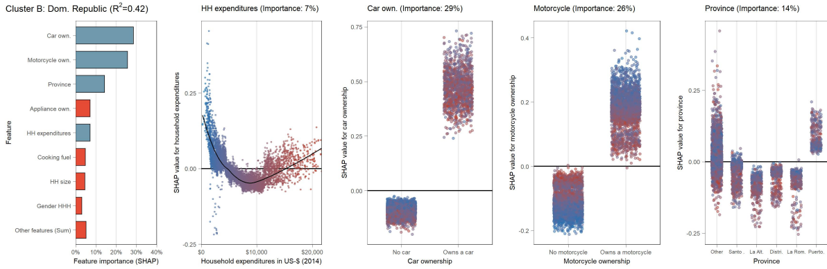
(B.9.53) Partial dependence plot (SHAP) for Dominican Republic (cluster B)
