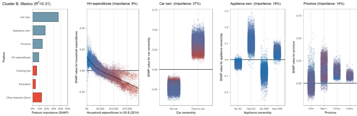
(B.9.59) Partial dependence plot (SHAP) for Mexico (cluster B)
