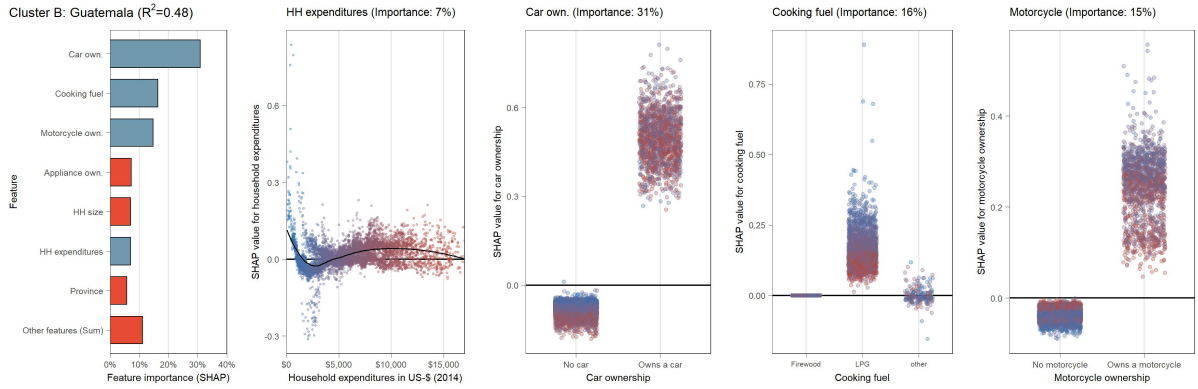
(B.9.56) Partial dependence plot (SHAP) for Guatemala (cluster B)
