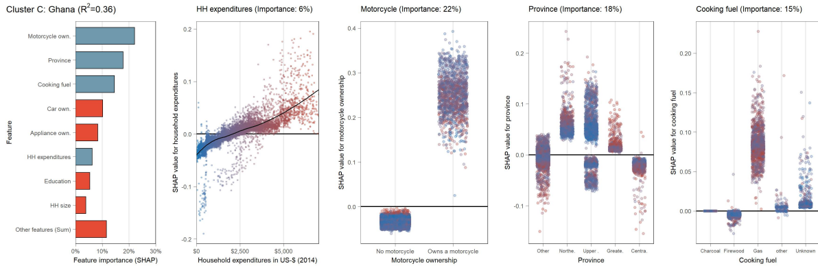
(B.9.70) Partial dependence plot (SHAP) for Ghana (cluster C)
