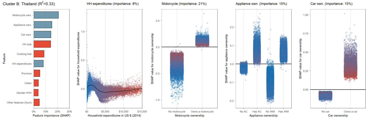
(B.9.62) Partial dependence plot (SHAP) for Thailand (cluster B)
