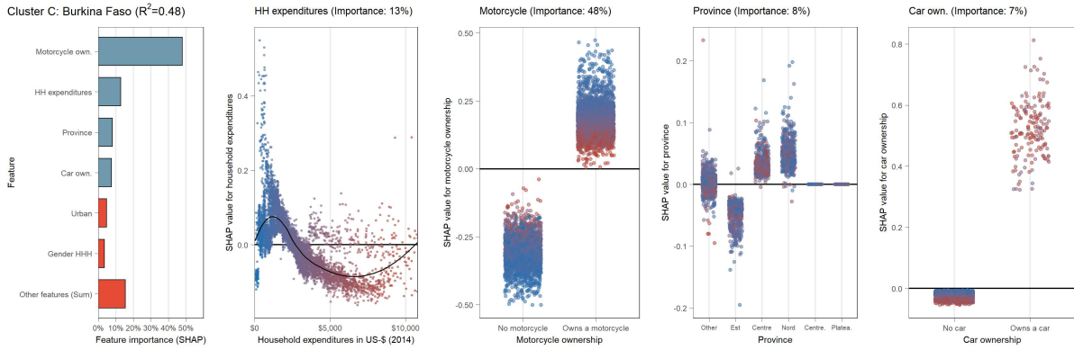
(B.9.68) Partial dependence plot (SHAP) for Burkina Faso (cluster C)
