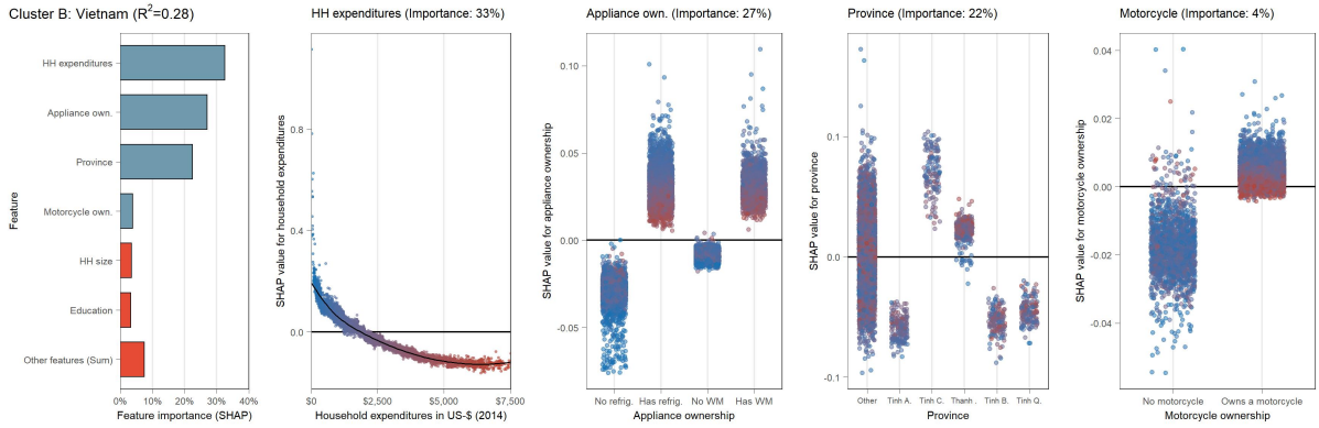
(B.9.65) Partial dependence plot (SHAP) for Vietnam (cluster B)
