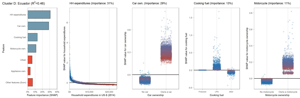
(B.9.79) Partial dependence plot (SHAP) for Ecuador (cluster D)
