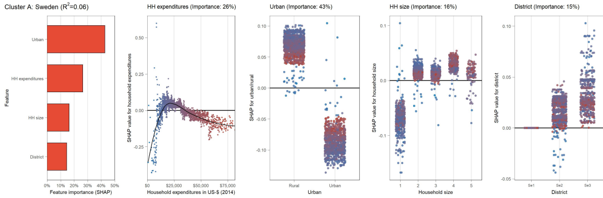
(B.9.49) Partial dependence plot (SHAP) for Sweden (cluster A)
