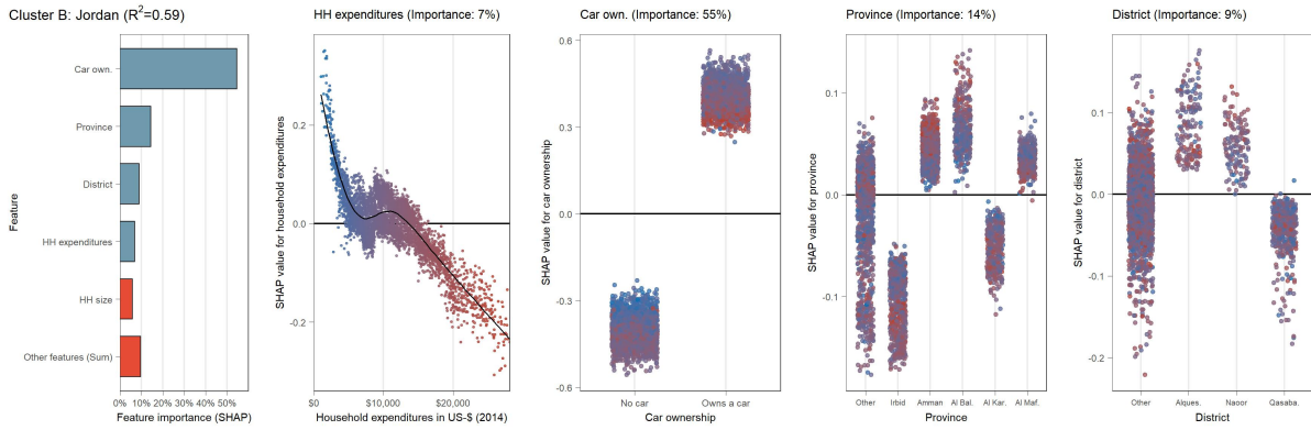
(B.9.58) Partial dependence plot (SHAP) for Jordan (cluster B)
