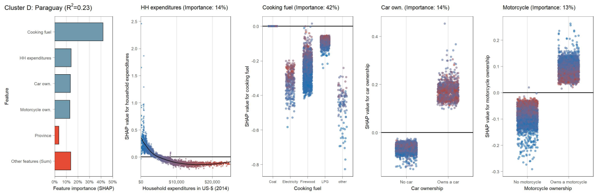
(B.9.83) Partial dependence plot (SHAP) for Paraguay (cluster D)
