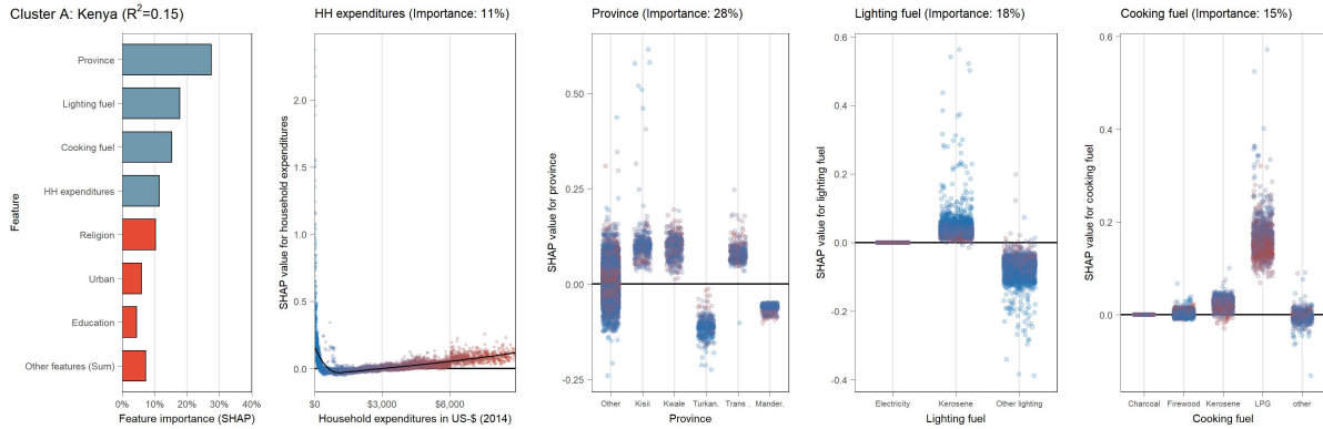
(B.9.29) Partial dependence plot (SHAP) for Kenya (cluster A)
