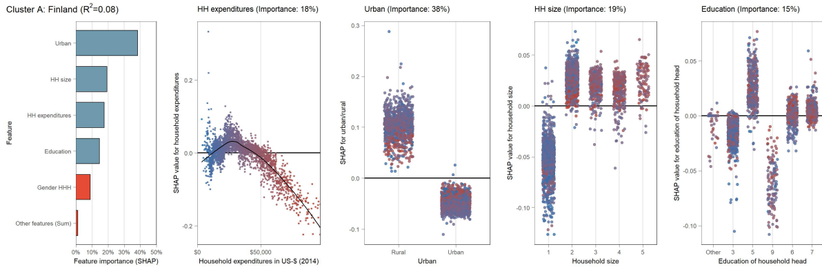
(B.9.19) Partial dependence plot (SHAP) for Finland (cluster A)
