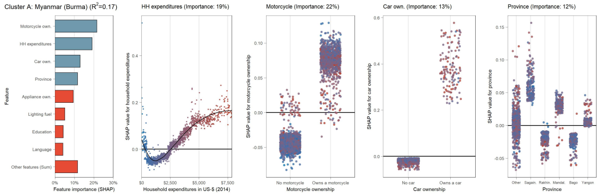
(B.9.37) Partial dependence plot (SHAP) for Myanmar (cluster A)
