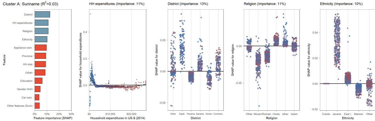
(B.9.47) Partial dependence plot (SHAP) for Suriname (cluster A)
