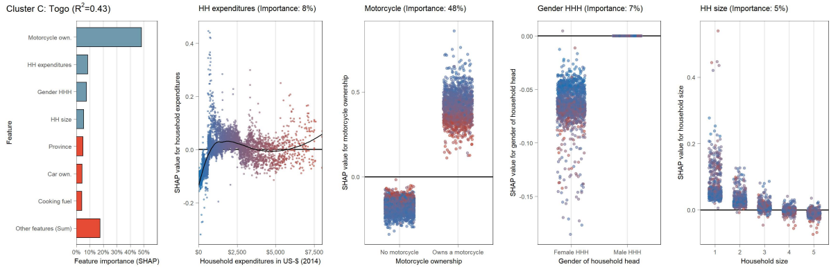
(B.9.77) Partial dependence plot (SHAP) for Togo (cluster C)
