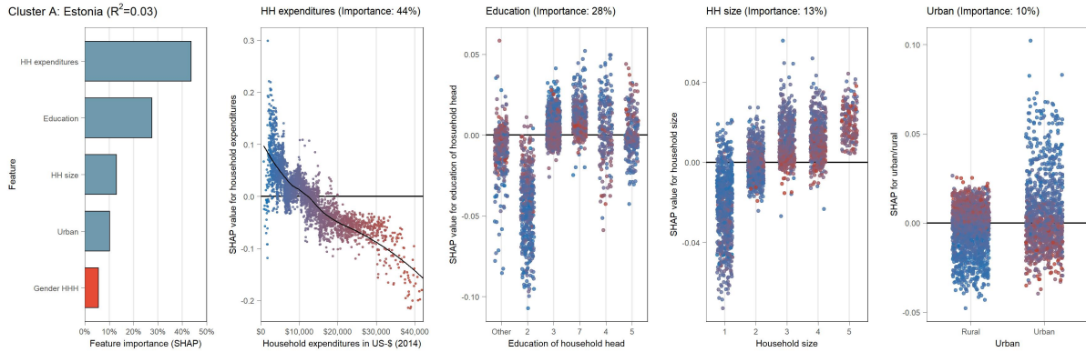
(B.9.17) Partial dependence plot (SHAP) for Estonia (cluster A)
