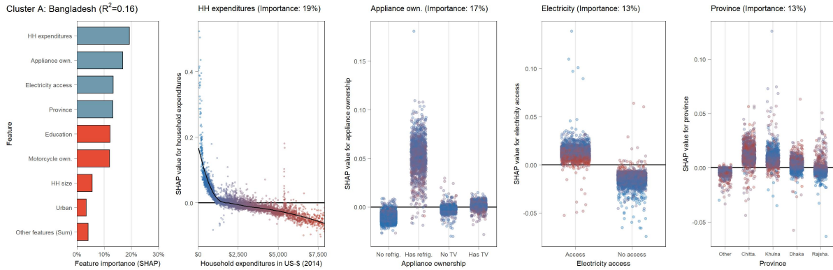
(B.9.5) Partial dependence plot (SHAP) for Bangladesh (cluster A)
