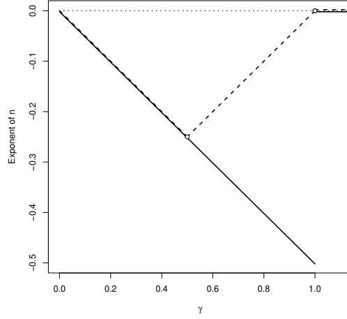
Figure 4.1: Exponent f(\gamma) of n as a function of \gamma for \|\boldsymbol{\theta}^{(n)} - \boldsymbol{\theta}^*\|_2 = O_{\mathbb{P}}(n^{f(\gamma)}) (solid line) from Theorem 7, \min_{0 \leq i \leq n} \|\boldsymbol{\theta}^{(i)} - \boldsymbol{\theta}^*\|_2 = O_{\mathbb{P}}(n^{f(\gamma)}) (dashed line) from Theorem 6, and \max_{0 \leq i \leq n} \|\boldsymbol{\theta}^{(i)} - \boldsymbol{\theta}^*\|_2 = O_{\mathbb{P}}(n^{f(\gamma)}) (dotted line) from Corollary 2; the empty points represent the presence of logarithmic terms or the coexistence of different convergence rates not depending on \gamma .
