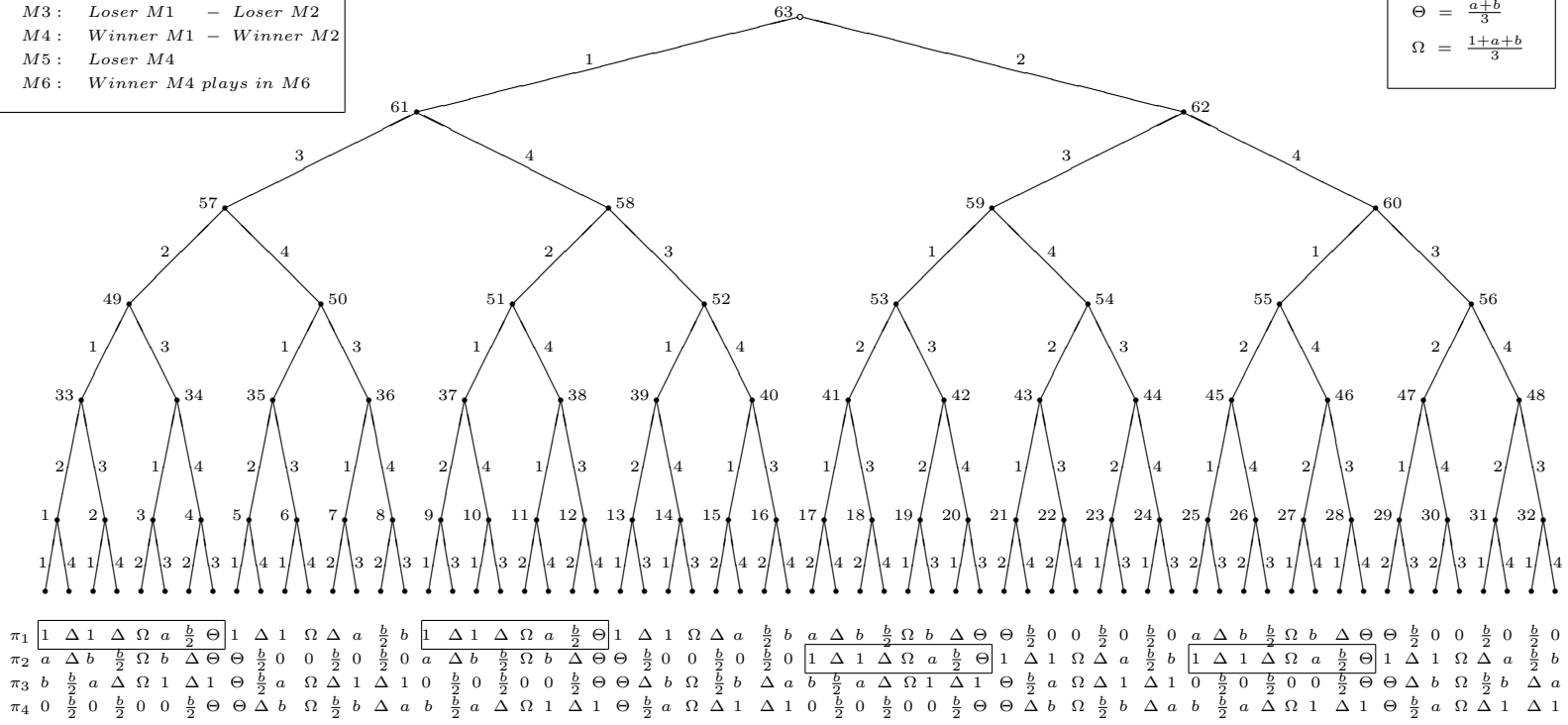
Figure 11: Game tree for LLL 4 : in boxes find payoff sequence A
