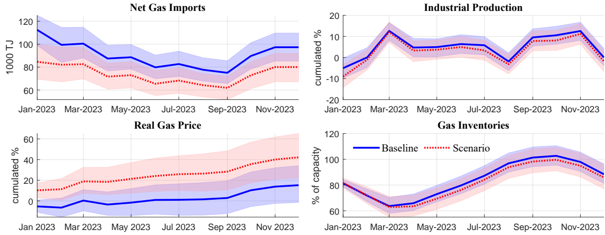
Figure 7: Conditional forecasts for a disruption of Europipe I and II in January 2023
