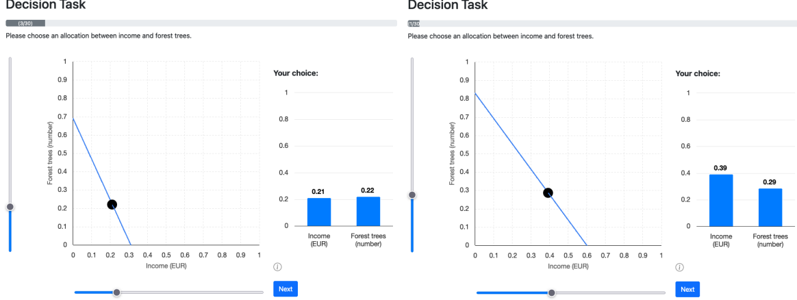
Figure 2: Illustrations of the experimental tasks.
