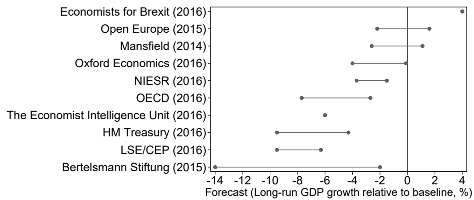
Figure C1: Long-run Forecasts
