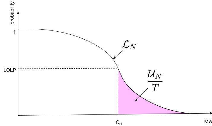
Figure 12: Inverted equivalent load duration curve and expected energy unserved
