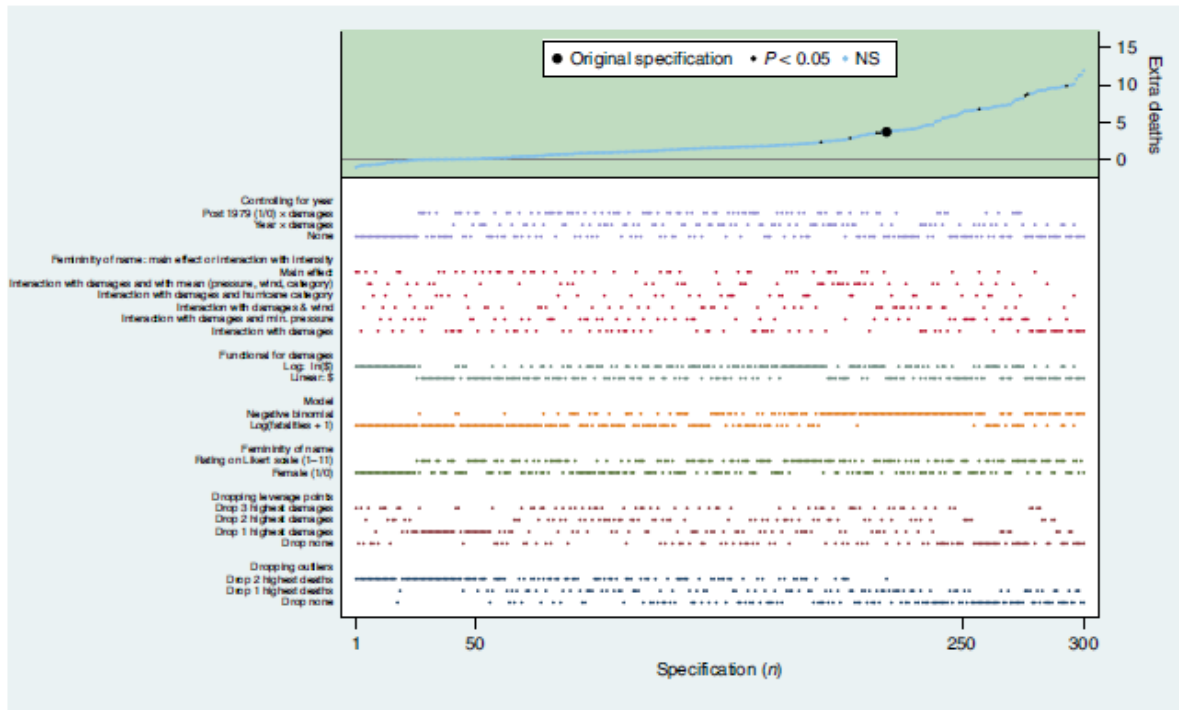
Figure 2: Specification Curve
