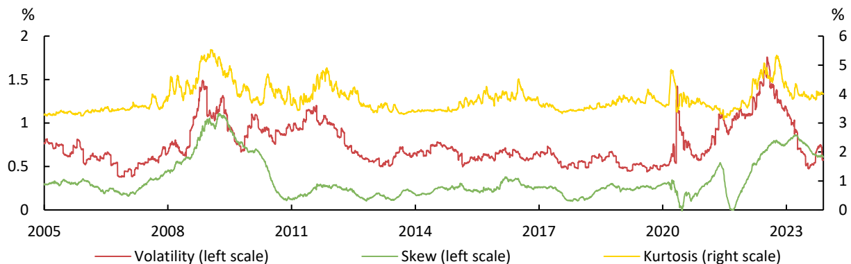
Chart 11: Risks around forecast inflation (%)
