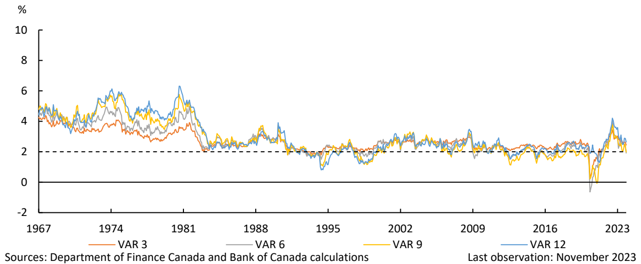
Chart 7: Augmenting the model-implied 10-year inflation expectations with survey data
