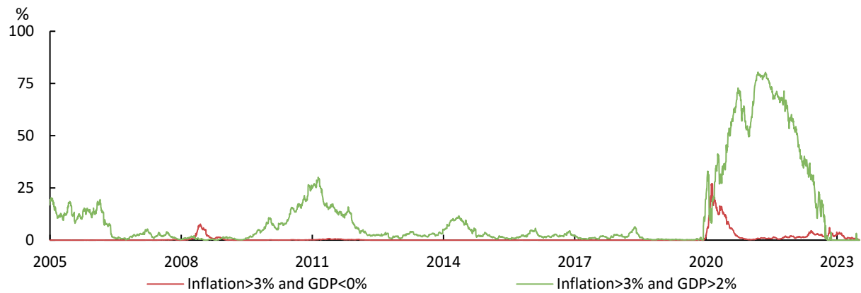
Chart 13: Joint probability of high inflation/strong growth, and high inflation/slow growth
