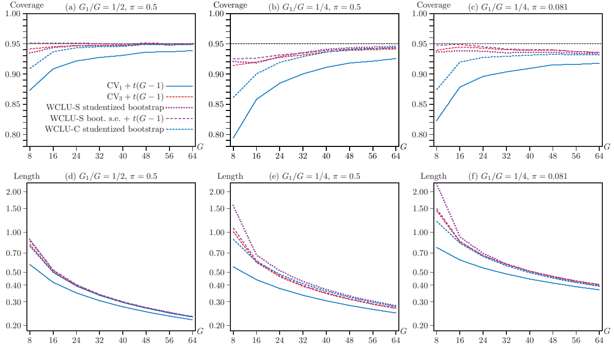
Figure 9: Performance of several confidence intervals as function of G
