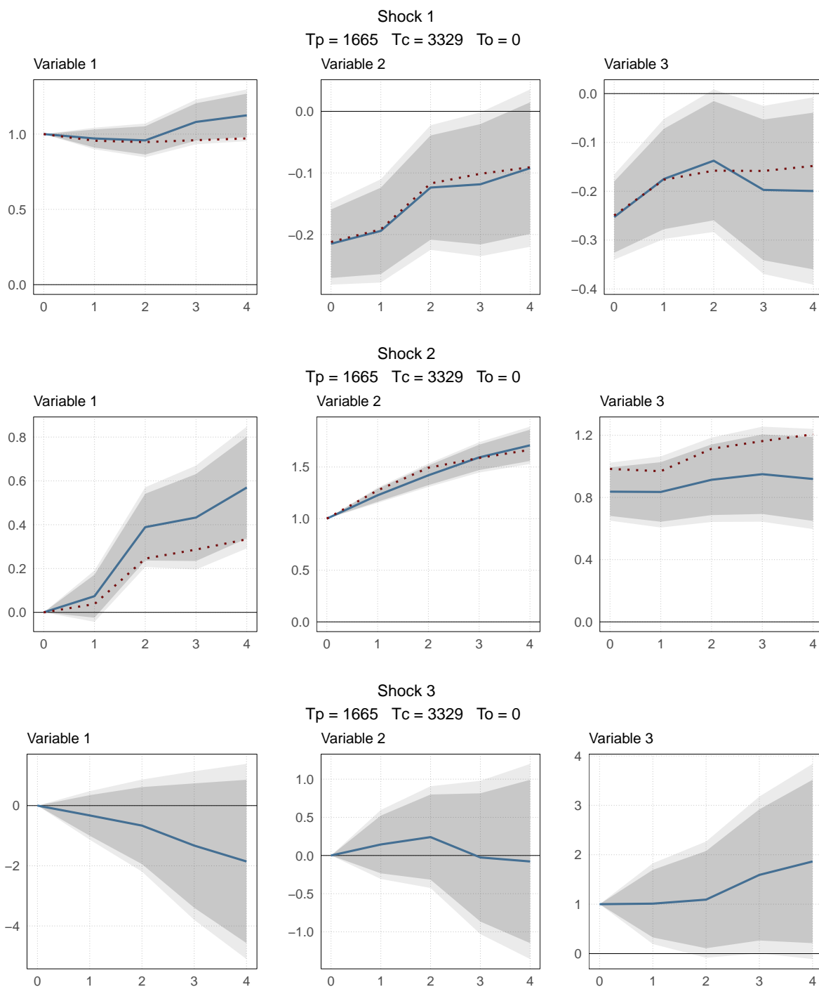
Fig. 5: Impulse responses for simulated data E = 2
