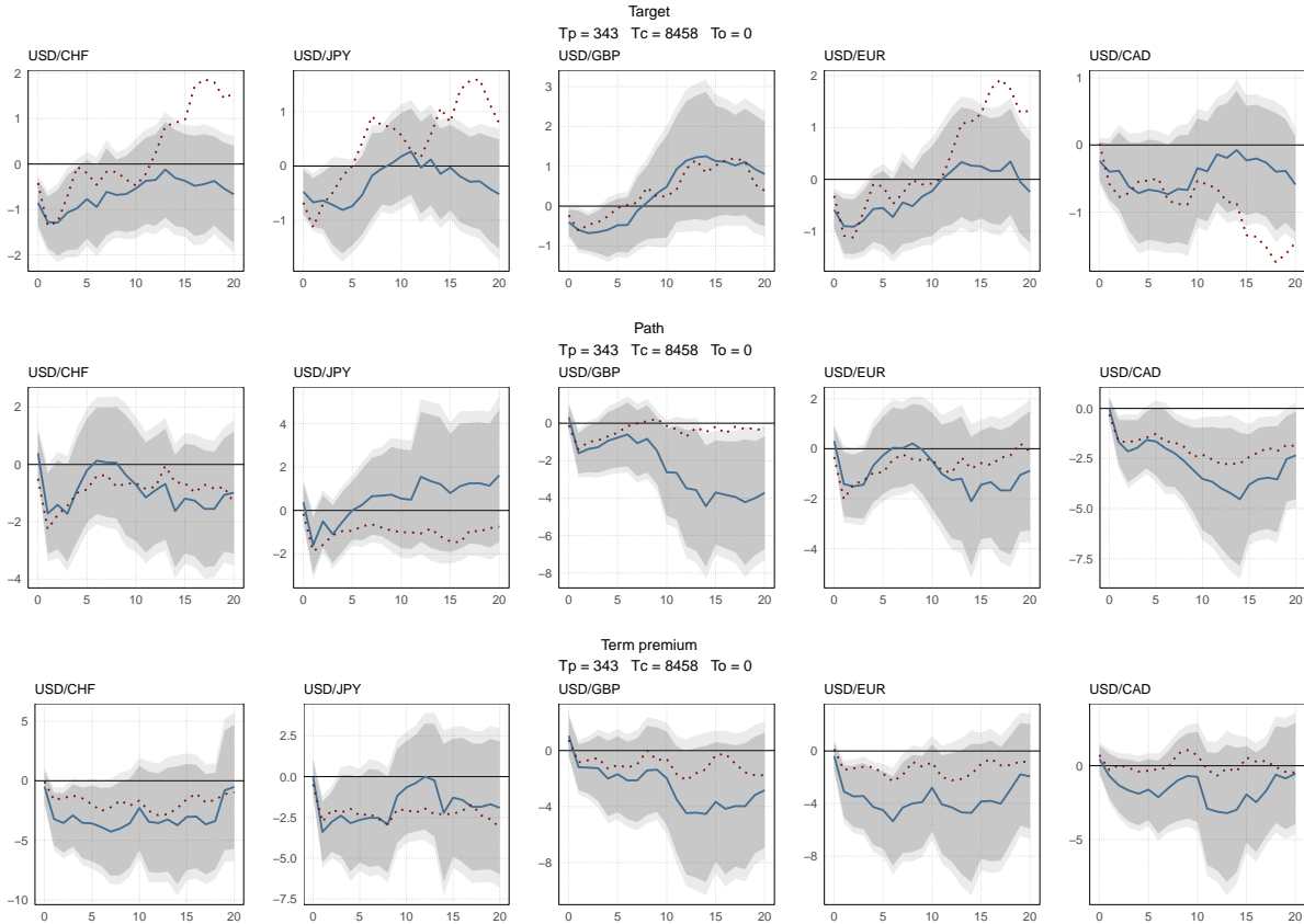
Fig. 4: Impulse responses of bilateral exchange rates
