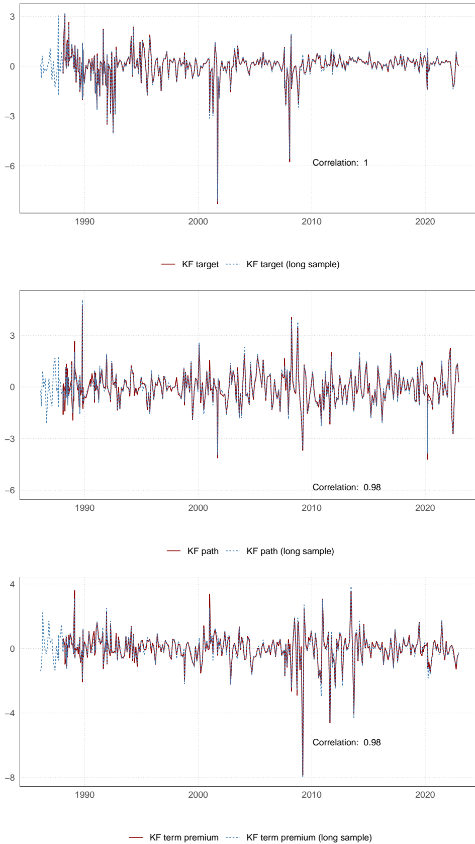
Fig. 13: Heteroscedasticity-based shocks starting in 1986
