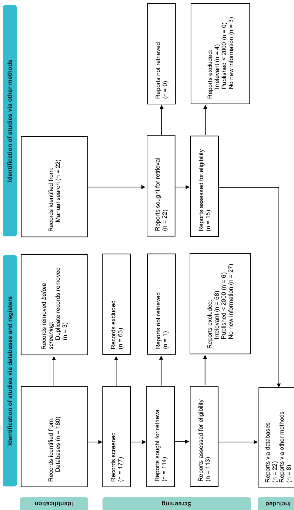
Figure 2 PRISMA diagram
