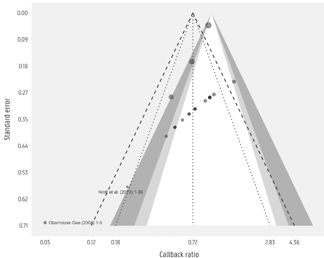
Figure B5. Contour-enhanced funnel plot: 19 to 36 months of unemployment
