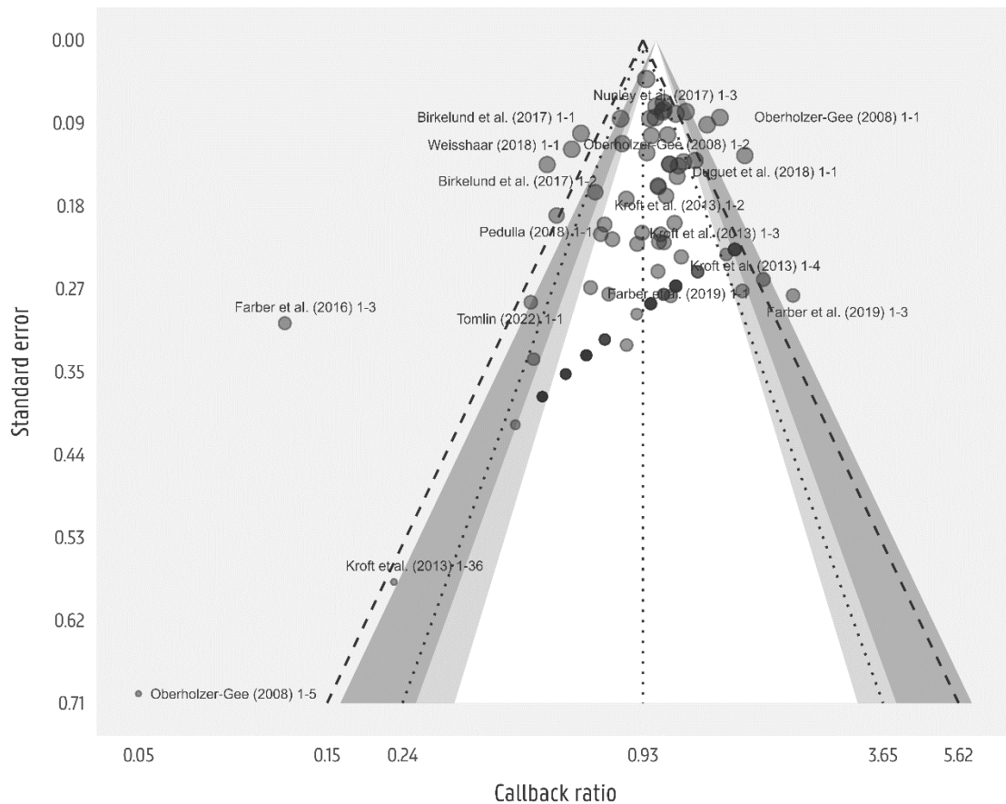
Figure B1. Contour-enhanced funnel plot: all treatment effects
