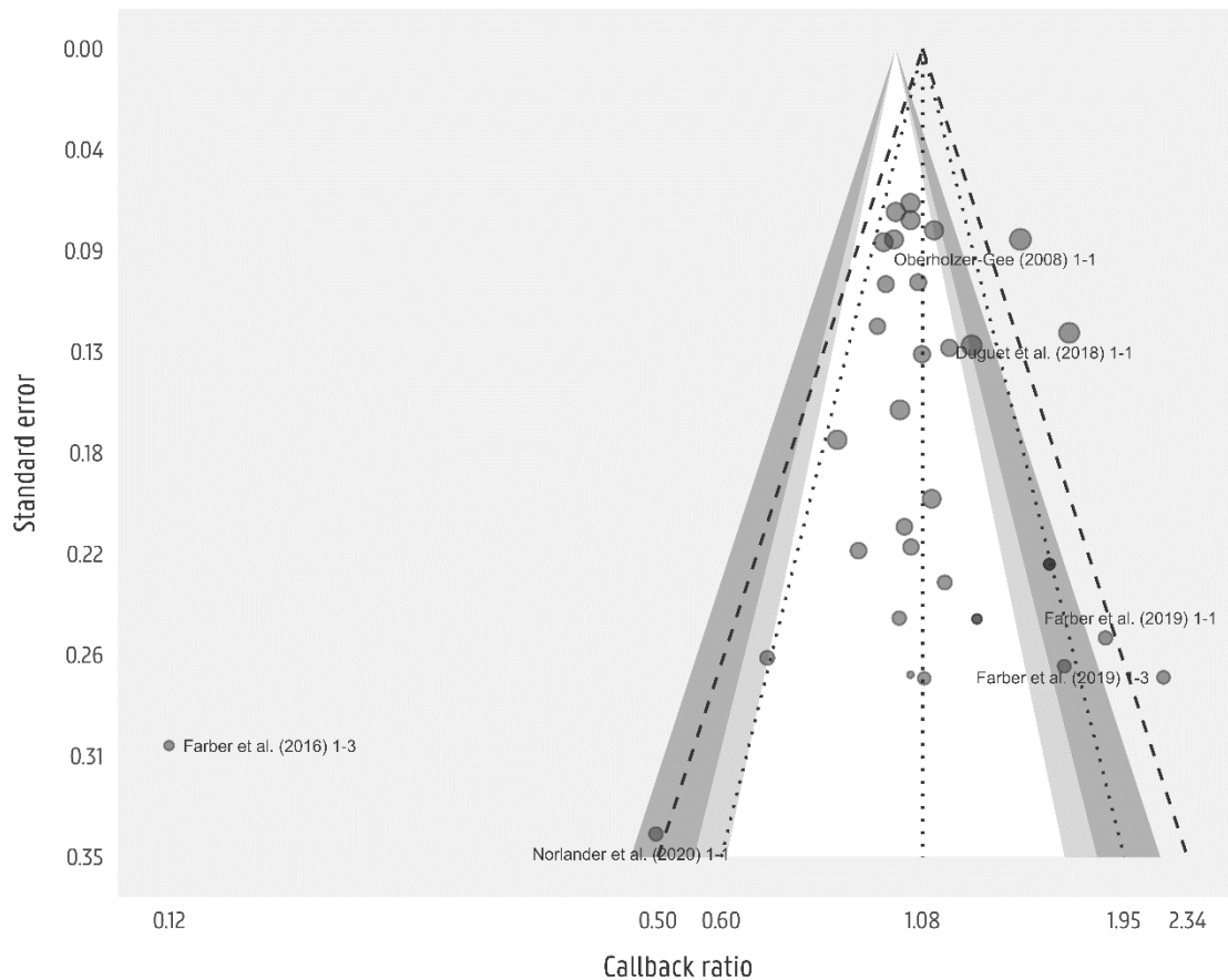
Figure B2. Contour-enhanced funnel plot: 1 to 6 months of unemployment
