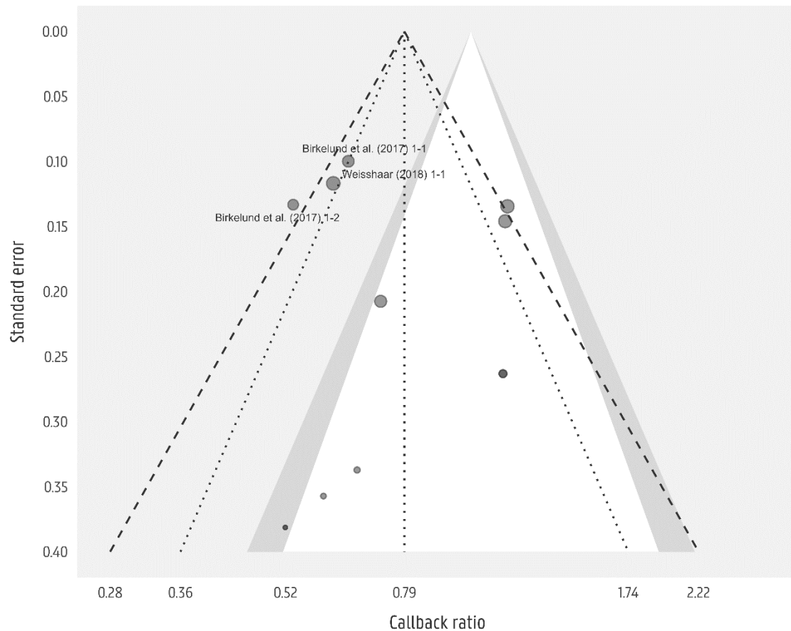
Figure B4. Contour-enhanced funnel plot: 13 to 18 months of unemployment
