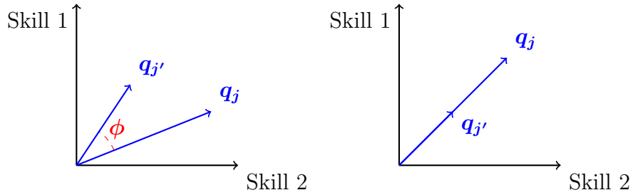
Figure 2: Illustration of distance between two occupations j and j' for K = 2
