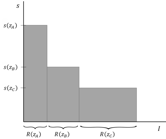
Figure 1: Optimal surplus s as a function of total research cost I
