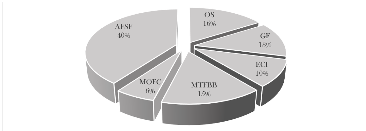
Figure 3. Percentage distribution land space in the Niger Delta.
